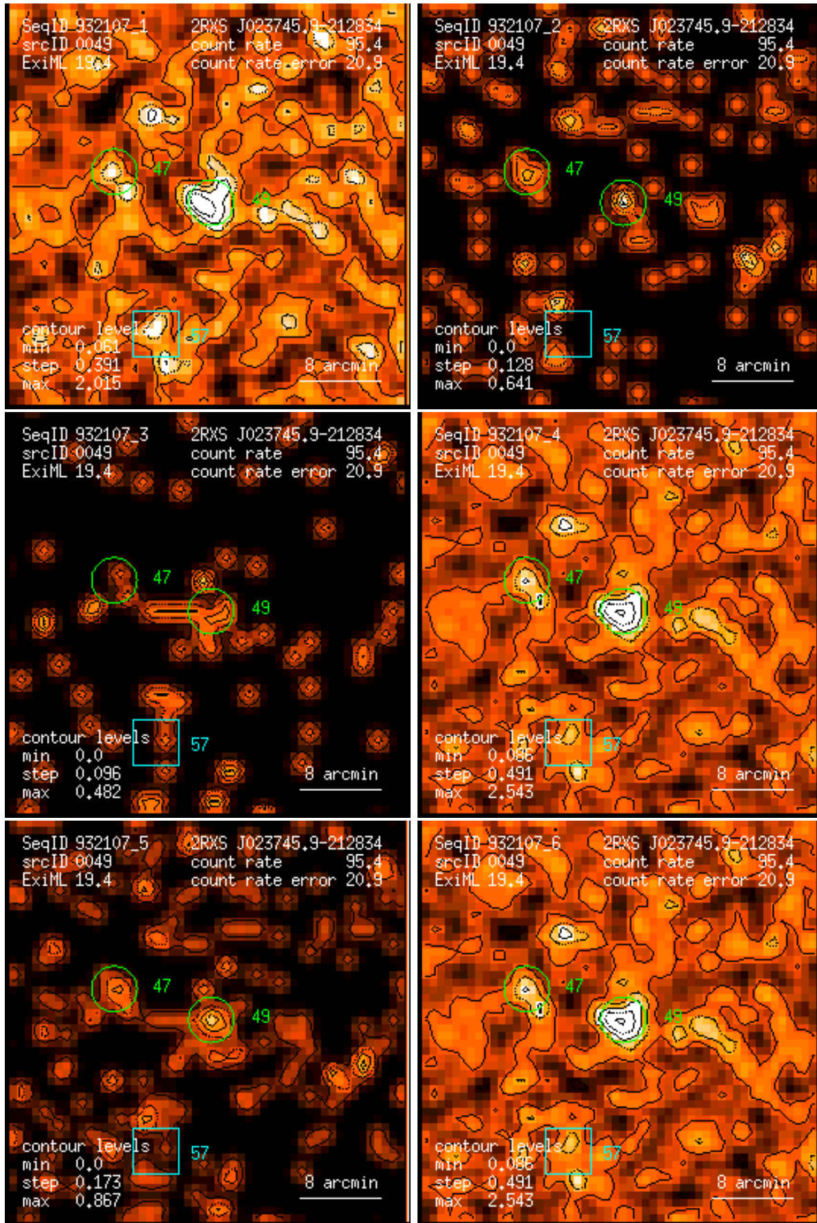
Figure 49: RASS 932107: detection 0049: band rate images, Gaussian filter: (1) PSPC channels 11 – 41, (2) 52 – 90, (3) 91 – 201, (4) 11 – 235, (5) 52 – 201, (6) 11 – 201. Broad band rates in counts/ks. Band rate contour levels in counts/ks/arcmin 2 .
