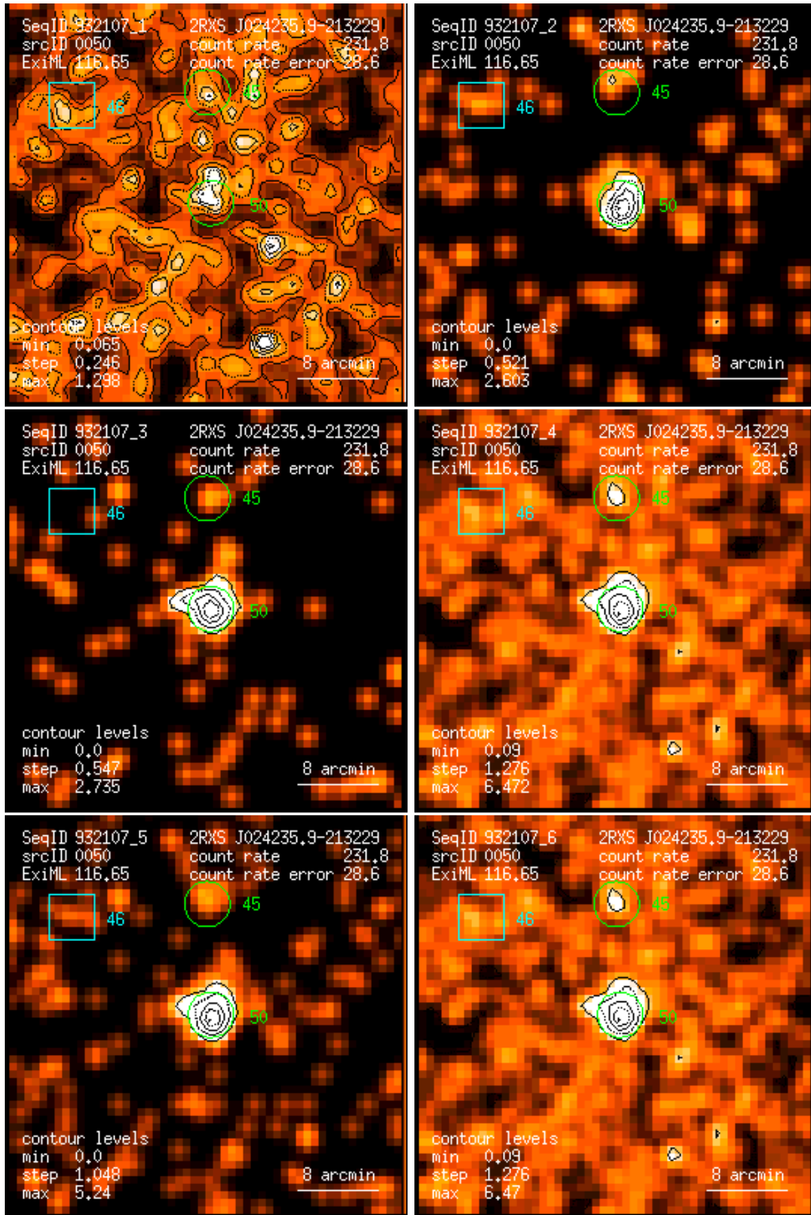
Figure 50: RASS 932107: detection 0050: band rate images, Gaussian filter: (1) PSPC channels 11 – 41, (2) 52 – 90, (3) 91 – 201, (4) 11 – 235, (5) 52 – 201, (6) 11 – 201. Broad band rates in counts/ks. Band rate contour levels in counts/ks/arcmin 2 .
