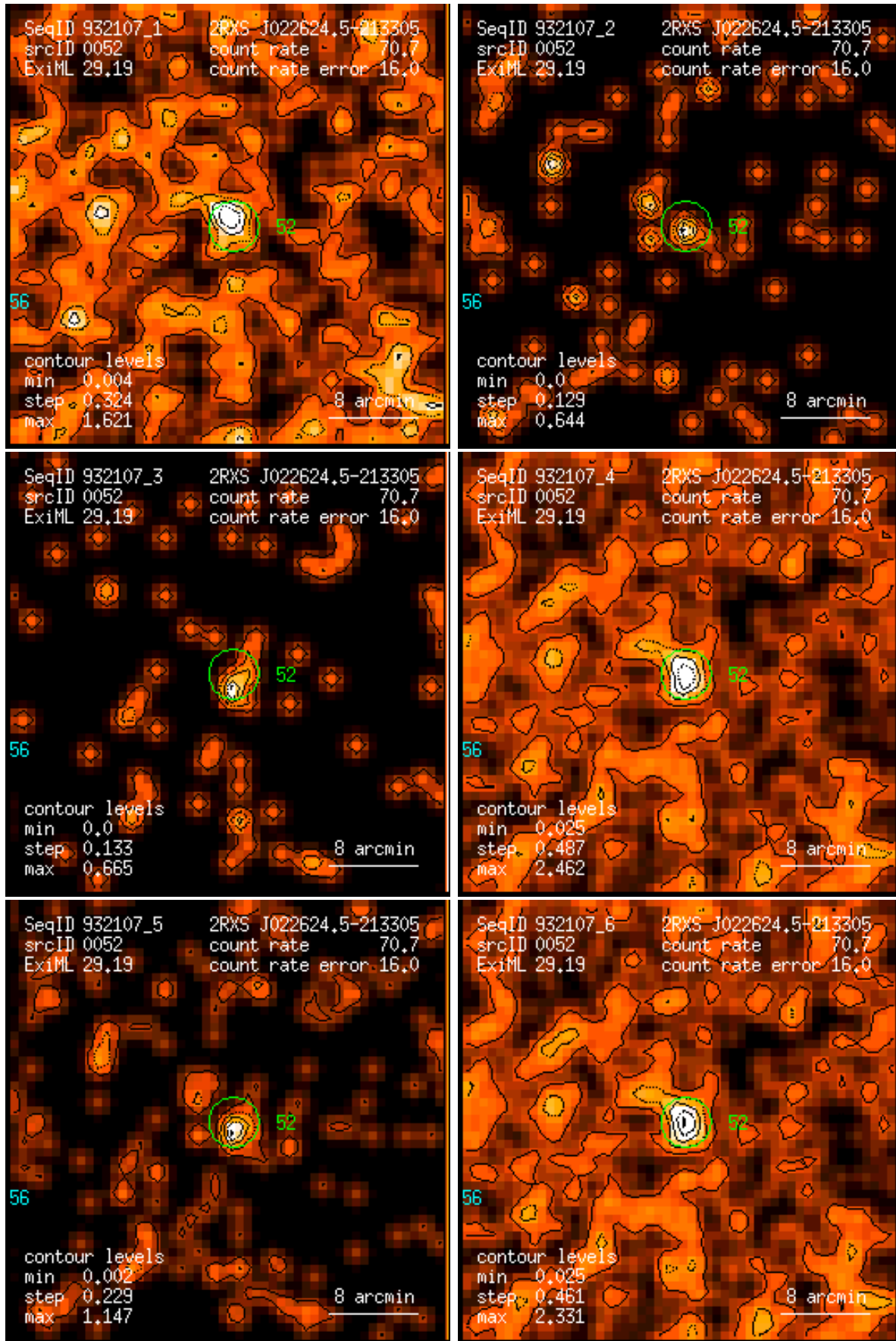
Figure 52: RASS 932107: detection 0052: band rate images, Gaussian filter: (1) PSPC channels 11 – 41, (2) 52 – 90, (3) 91 – 201, (4) 11 – 235, (5) 52 – 201, (6) 11 – 201. Broad band rates in counts/ks. Band rate contour levels in counts/ks/arcmin 2 .
