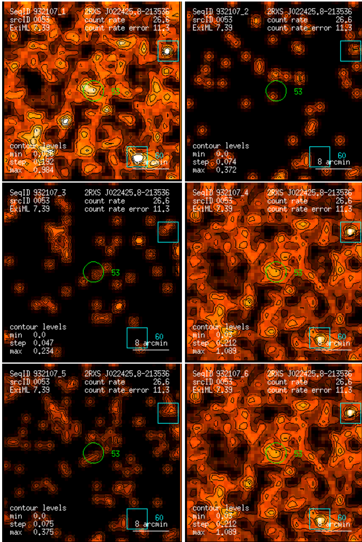
Figure 53: RASS 932107: detection 0053: band rate images, Gaussian filter: (1) PSPC channels 11 – 41, (2) 52 – 90, (3) 91 – 201, (4) 11 – 235, (5) 52 – 201, (6) 11 – 201. Broad band rates in counts/ks. Band rate contour levels in counts/ks/arcmin 2 .
