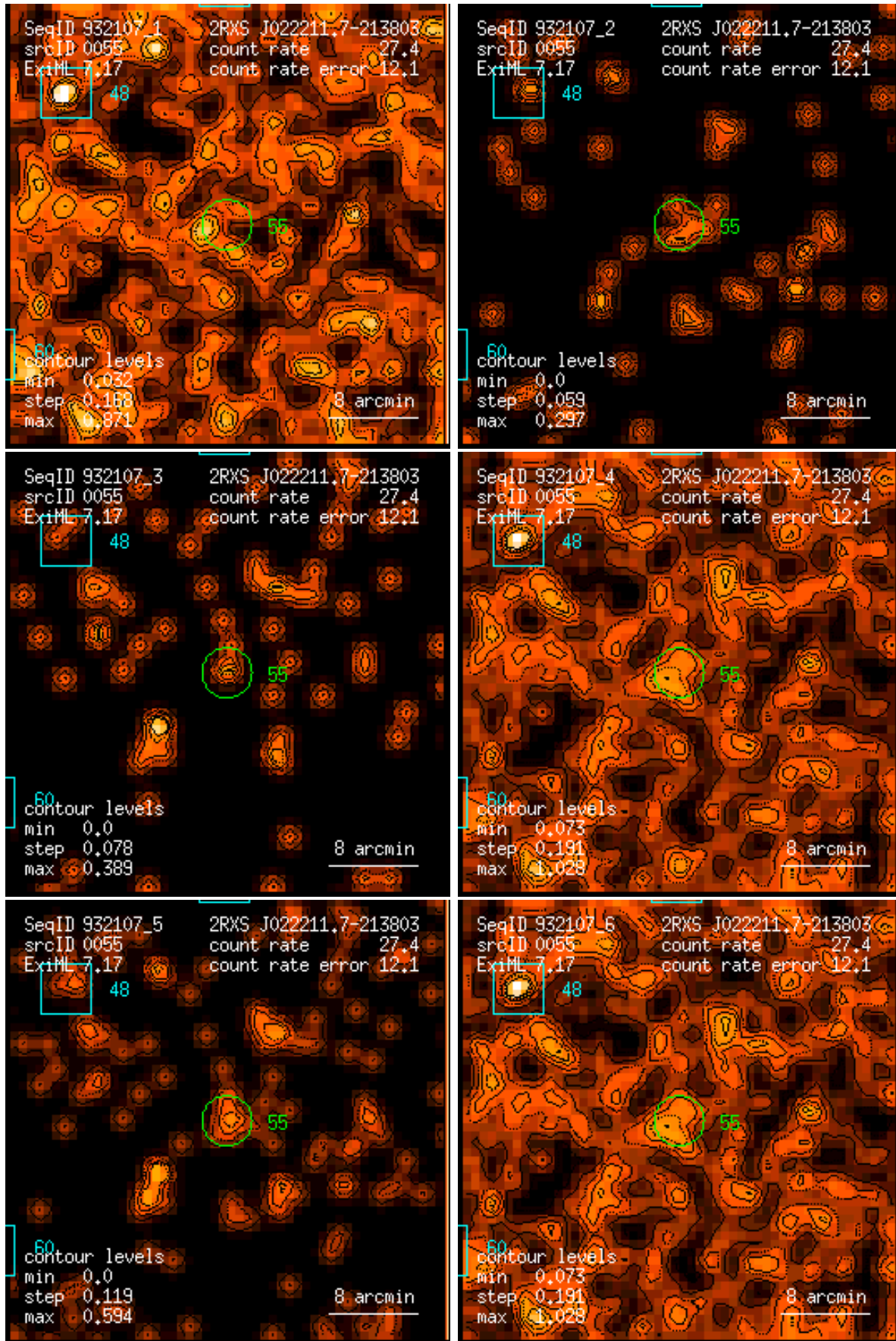
Figure 55: RASS 932107: detection 0055: band rate images, Gaussian filter: (1) PSPC channels 11 – 41, (2) 52 – 90, (3) 91 – 201, (4) 11 – 235, (5) 52 – 201, (6) 11 – 201. Broad band rates in counts/ks. Band rate contour levels in counts/ks/arcmin 2 .
