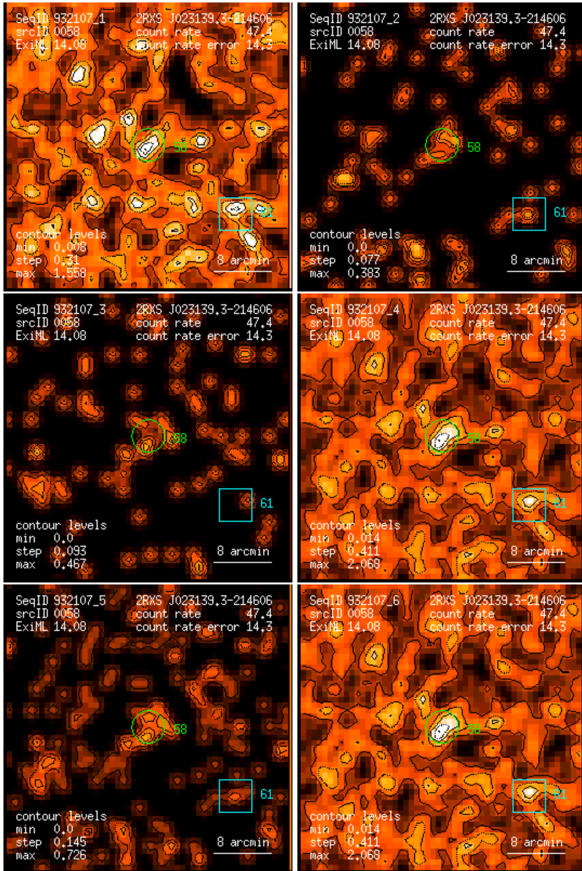
Figure 58: RASS 932107: detection 0058: band rate images, Gaussian filter: (1) PSPC channels 11 – 41, (2) 52 – 90, (3) 91 – 201, (4) 11 – 235, (5) 52 – 201, (6) 11 – 201. Broad band rates in counts/ks. Band rate contour levels in counts/ks/arcmin 2 .
