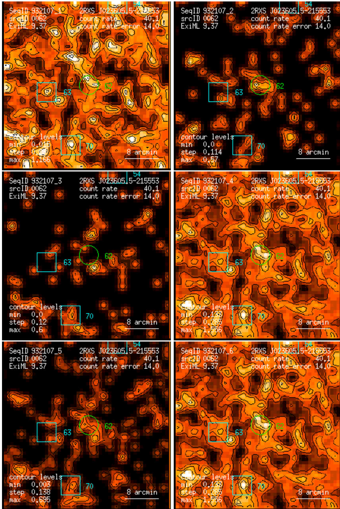
Figure 62: RASS 932107: detection 0062: band rate images, Gaussian filter: (1) PSPC channels 11 – 41, (2) 52 – 90, (3) 91 – 201, (4) 11 – 235, (5) 52 – 201, (6) 11 – 201. Broad band rates in counts/ks. Band rate contour levels in counts/ks/arcmin 2 .
