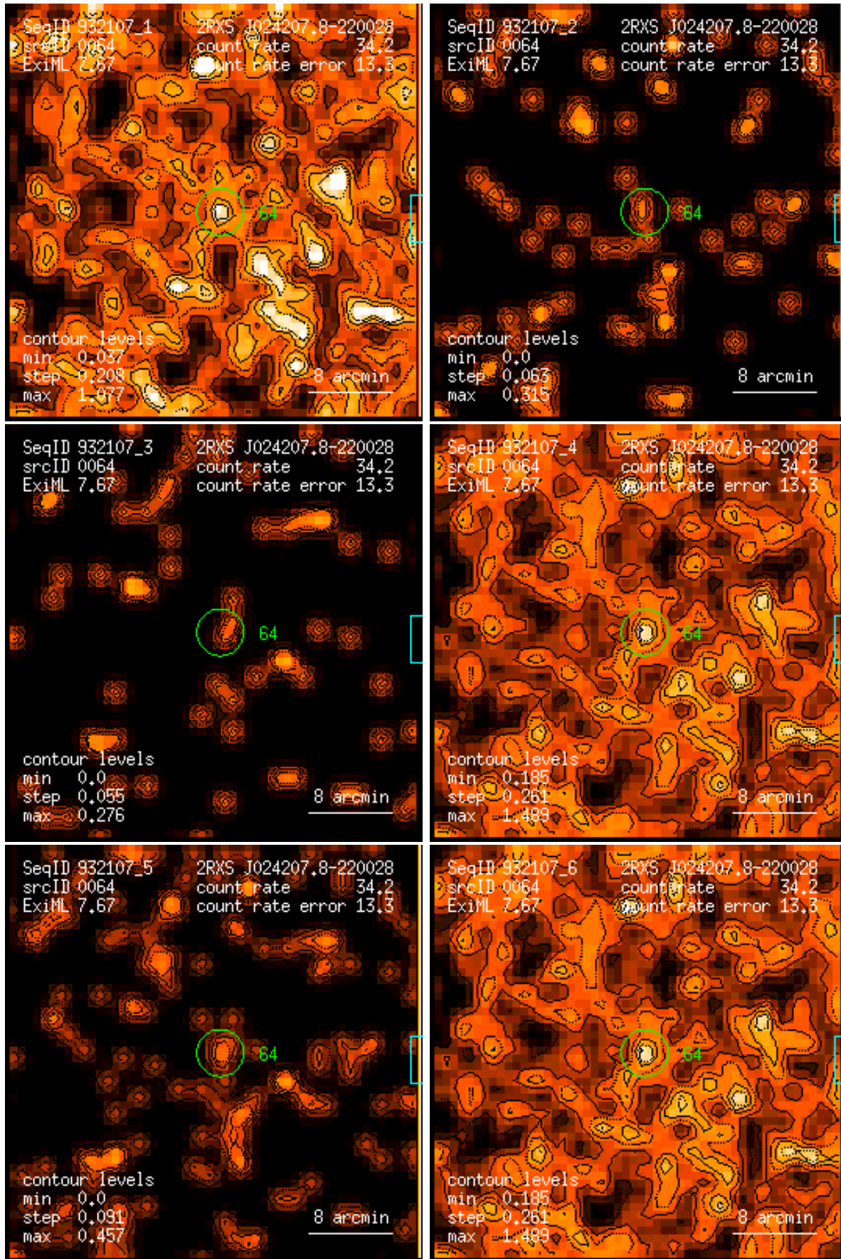
Figure 64: RASS 932107: detection 0064: band rate images, Gaussian filter: (1) PSPC channels 11 – 41, (2) 52 – 90, (3) 91 – 201, (4) 11 – 235, (5) 52 – 201, (6) 11 – 201. Broad band rates in counts/ks. Band rate contour levels in counts/ks/arcmin 2 .
