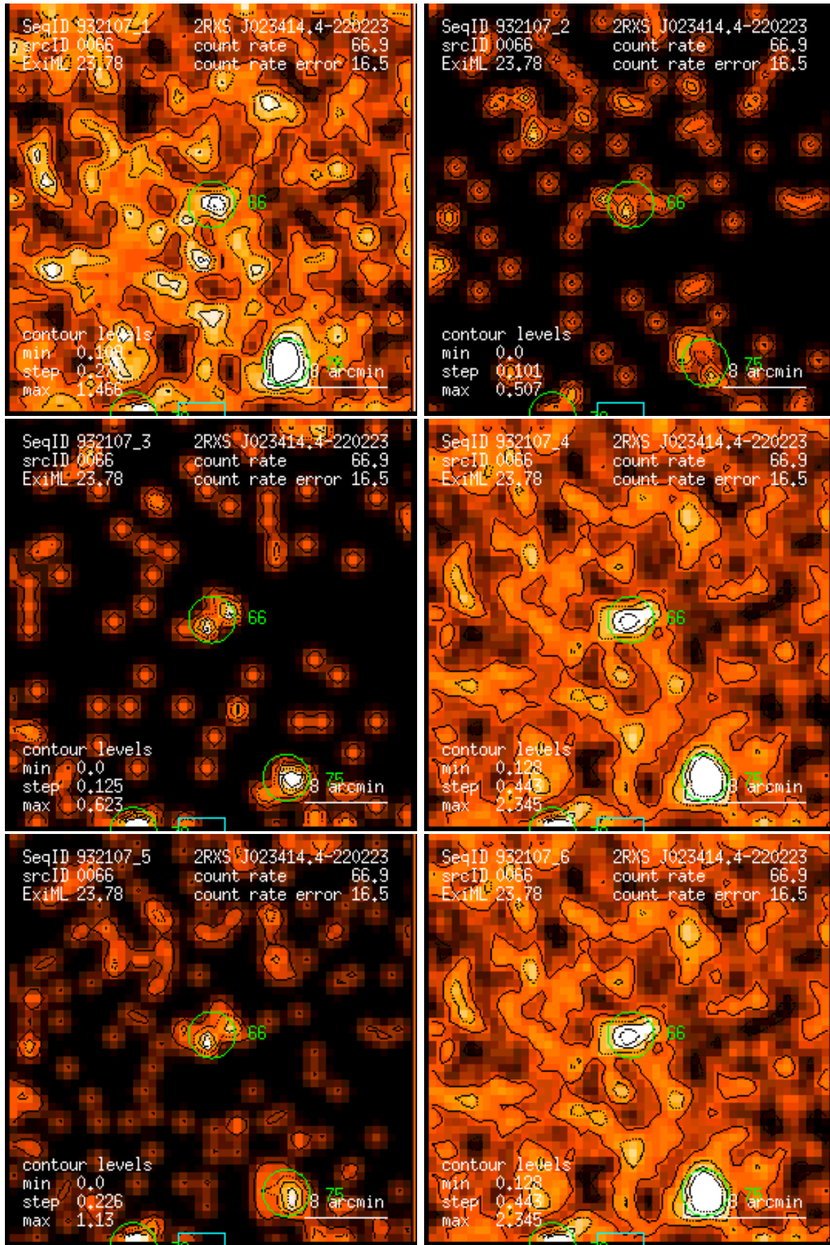
Figure 66: RASS 932107: detection 0066: band rate images, Gaussian filter: (1) PSPC channels 11 – 41, (2) 52 – 90, (3) 91 – 201, (4) 11 – 235, (5) 52 – 201, (6) 11 – 201. Broad band rates in counts/ks. Band rate contour levels in counts/ks/arcmin 2 .
