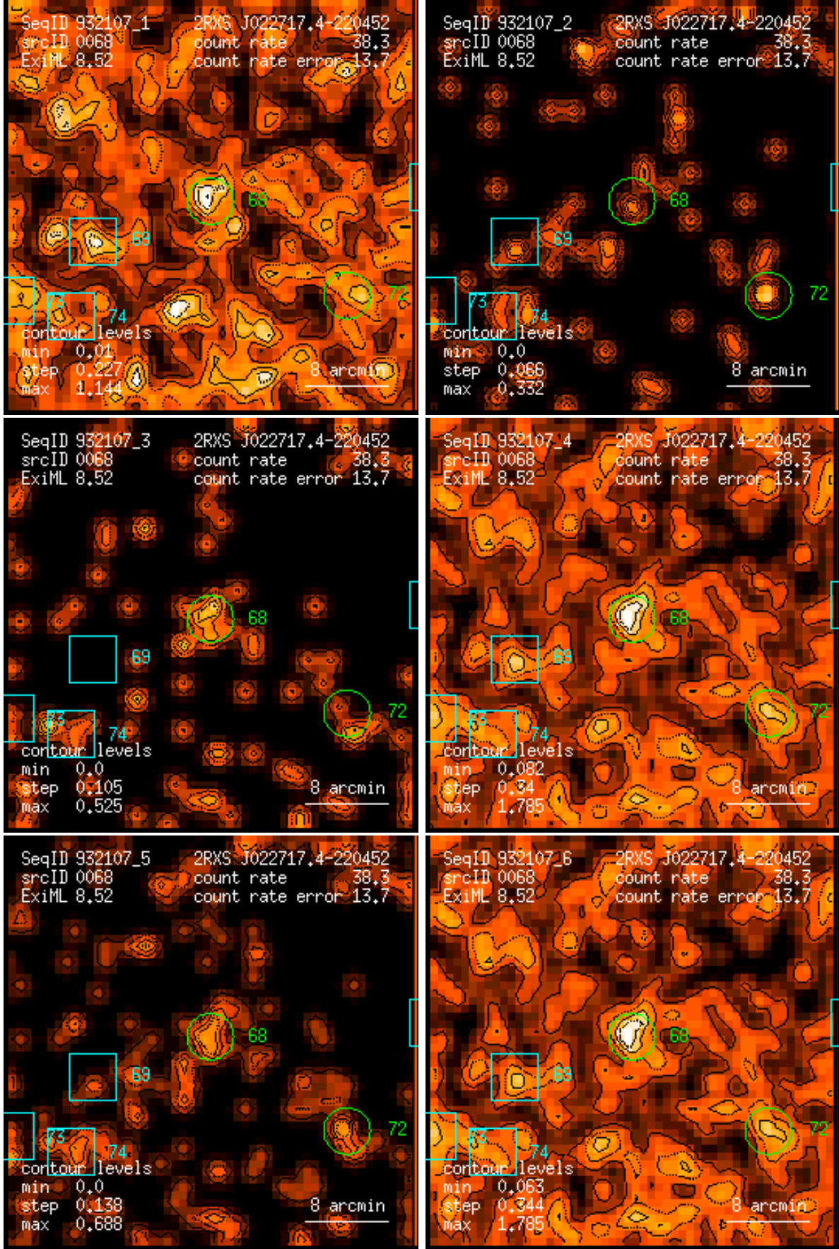
Figure 68: RASS 932107: detection 0068: band rate images, Gaussian filter: (1) PSPC channels 11 – 41, (2) 52 – 90, (3) 91 – 201, (4) 11 – 235, (5) 52 – 201, (6) 11 – 201. Broad band rates in counts/ks. Band rate contour levels in counts/ks/arcmin 2 .
