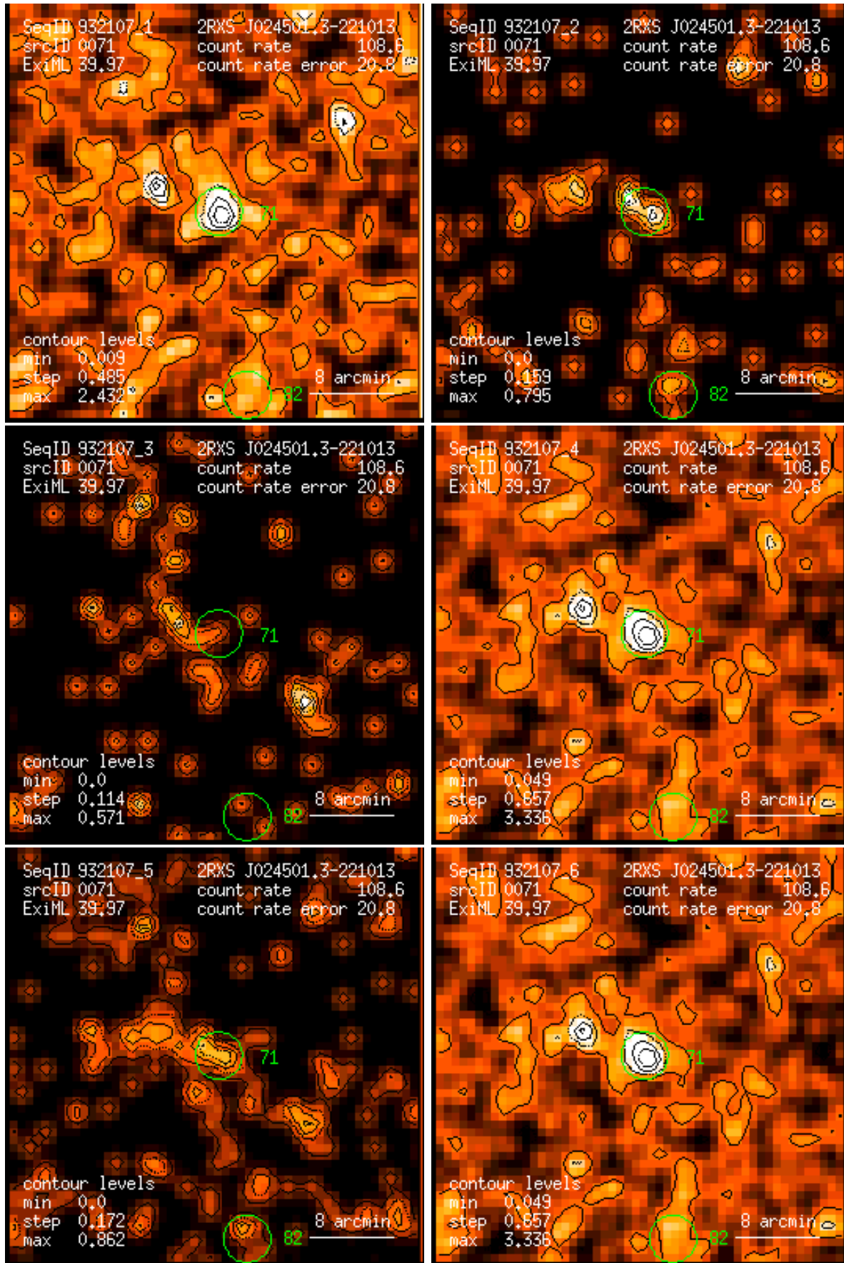
Figure 71: RASS 932107: detection 0071: band rate images, Gaussian filter: (1) PSPC channels 11 – 41, (2) 52 – 90, (3) 91 – 201, (4) 11 – 235, (5) 52 – 201, (6) 11 – 201. Broad band rates in counts/ks. Band rate contour levels in counts/ks/arcmin 2 .
