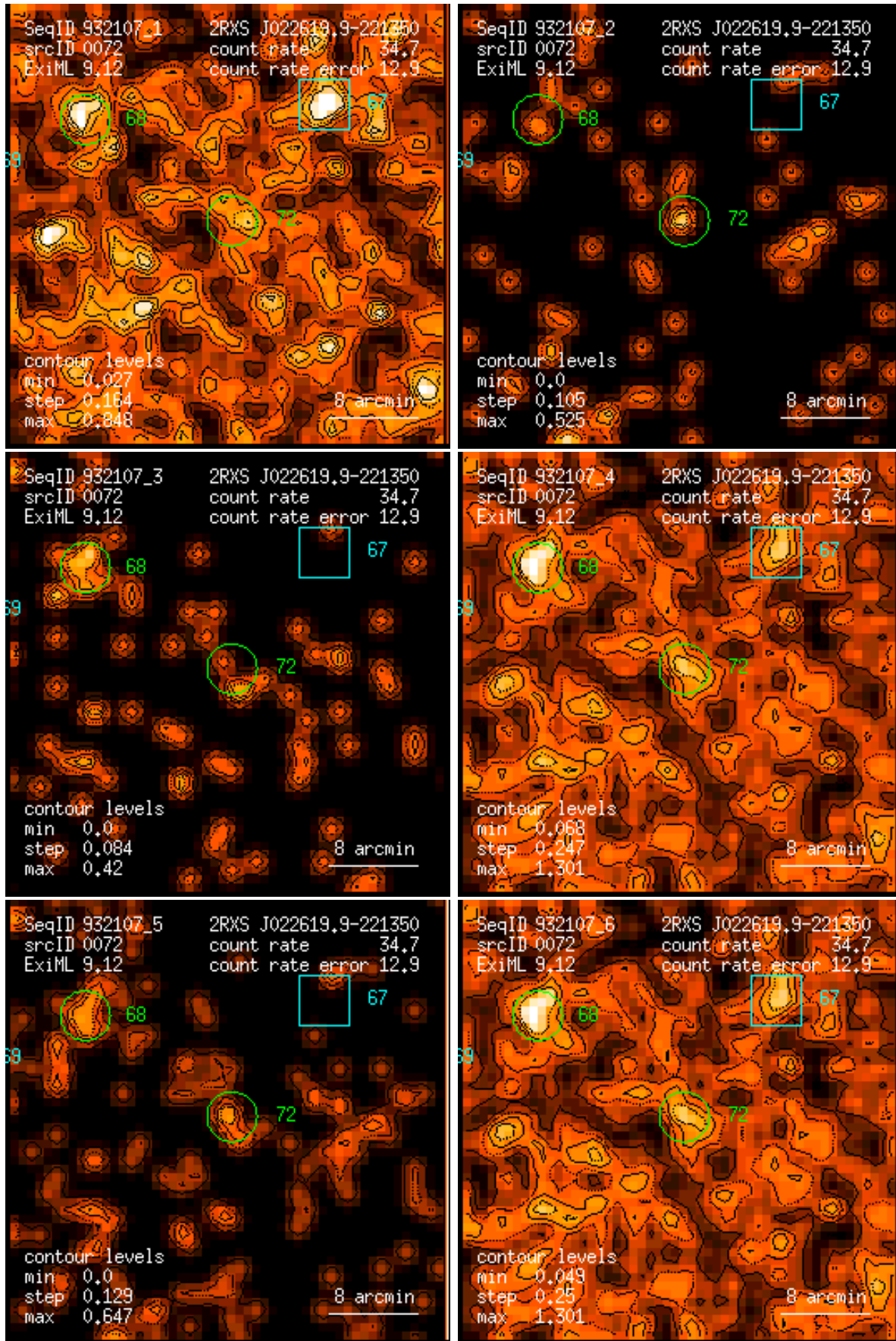
Figure 72: RASS 932107: detection 0072: band rate images, Gaussian filter: (1) PSPC channels 11 – 41, (2) 52 – 90, (3) 91 – 201, (4) 11 – 235, (5) 52 – 201, (6) 11 – 201. Broad band rates in counts/ks. Band rate contour levels in counts/ks/arcmin 2 .
