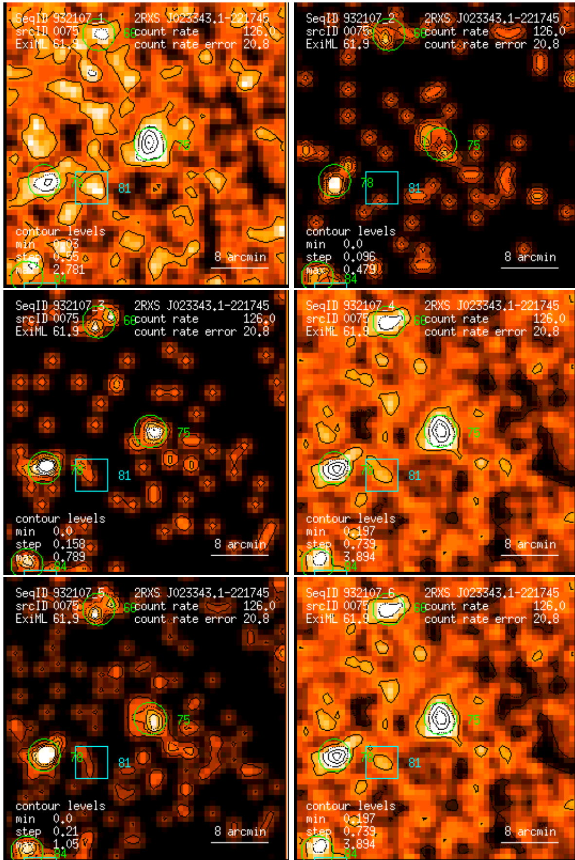
Figure 75: RASS 932107: detection 0075: band rate images, Gaussian filter: (1) PSPC channels 11 – 41, (2) 52 – 90, (3) 91 – 201, (4) 11 – 235, (5) 52 – 201, (6) 11 – 201. Broad band rates in counts/ks. Band rate contour levels in counts/ks/arcmin 2 .
