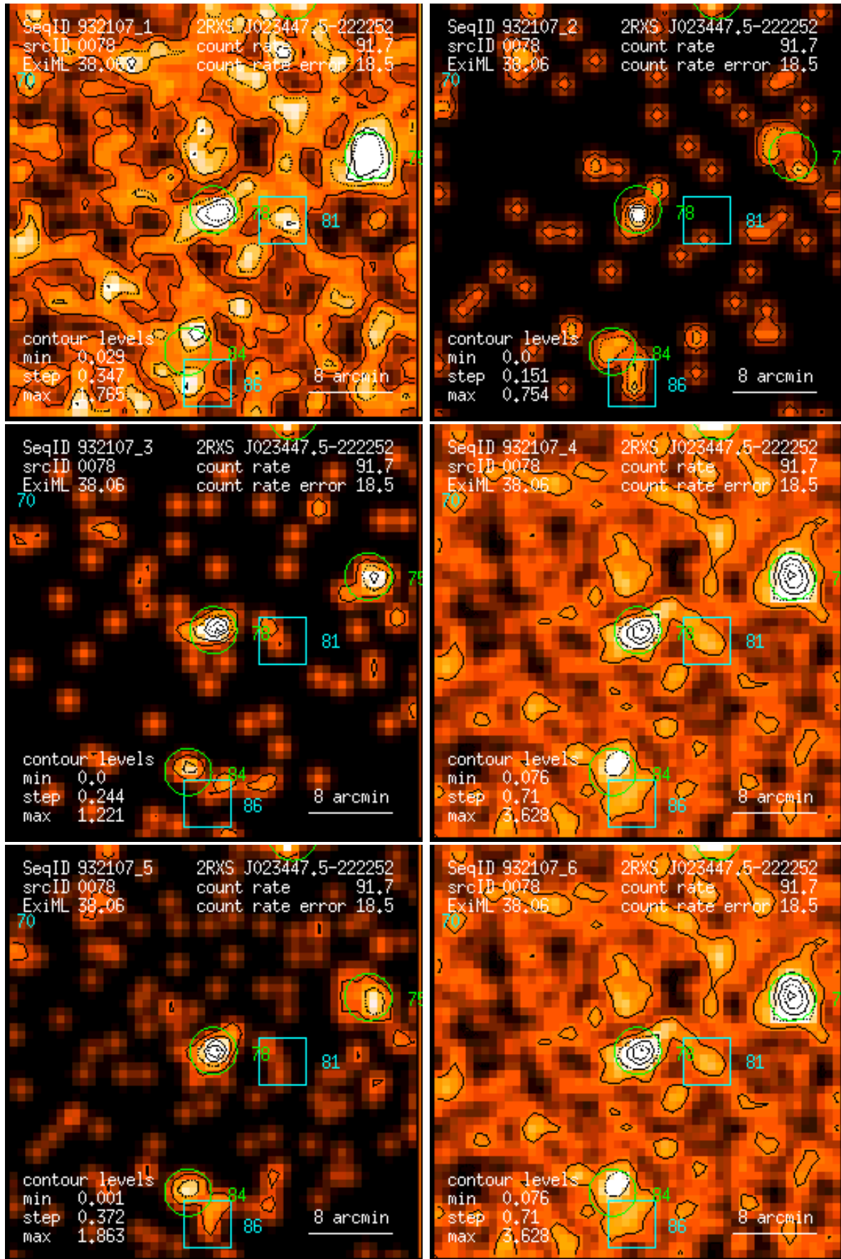
Figure 78: RASS 932107: detection 0078: band rate images, Gaussian filter: (1) PSPC channels 11 – 41, (2) 52 – 90, (3) 91 – 201, (4) 11 – 235, (5) 52 – 201, (6) 11 – 201. Broad band rates in counts/ks. Band rate contour levels in counts/ks/arcmin 2 .
