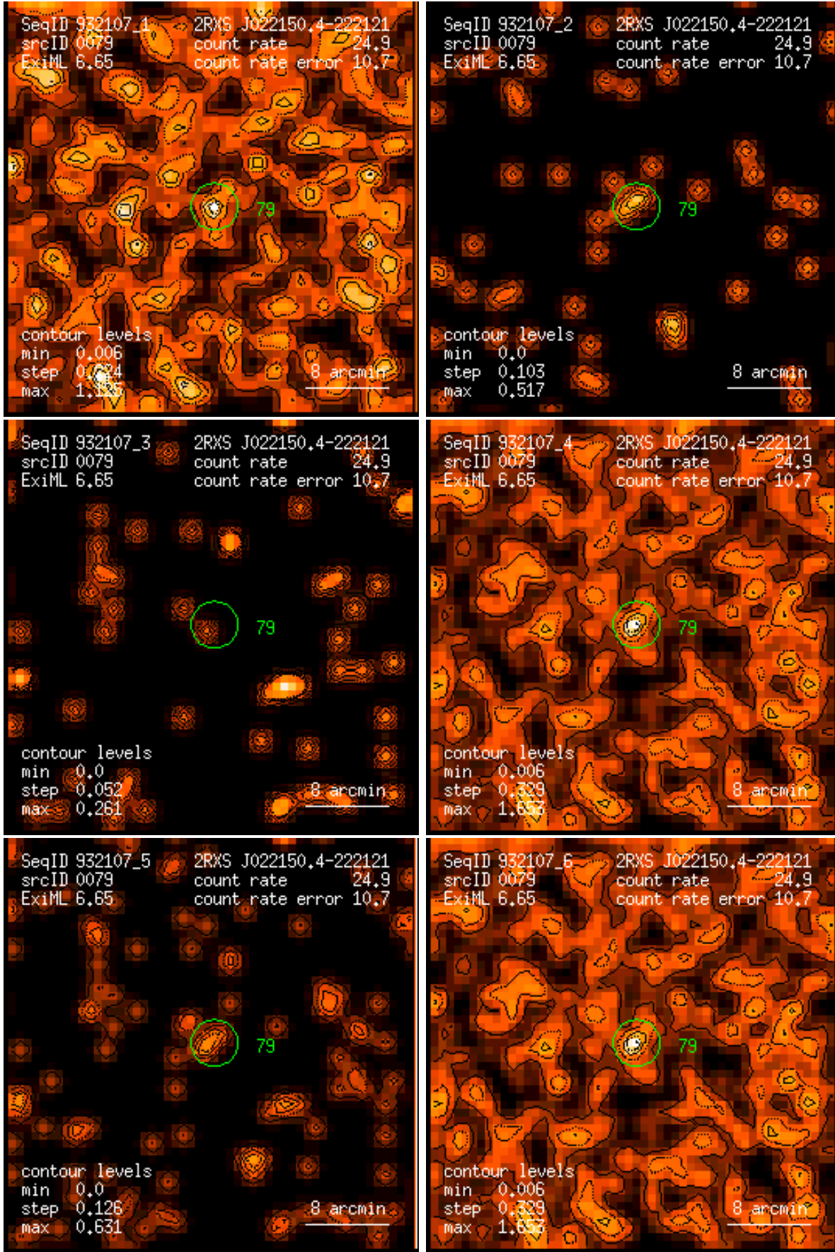
Figure 79: RASS 932107: detection 0079: band rate images, Gaussian filter: (1) PSPC channels 11 – 41, (2) 52 – 90, (3) 91 – 201, (4) 11 – 235, (5) 52 – 201, (6) 11 – 201. Broad band rates in counts/ks. Band rate contour levels in counts/ks/arcmin 2 .
