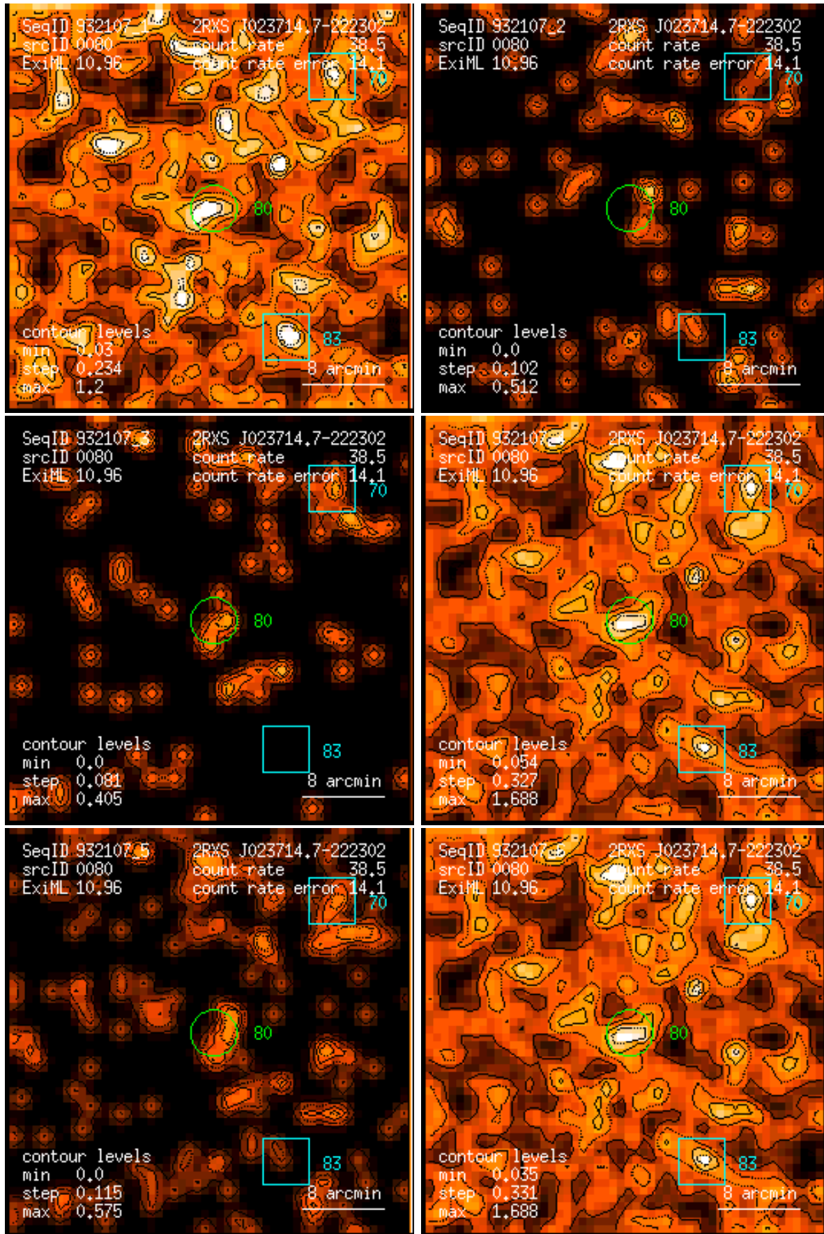
Figure 80: RASS 932107: detection 0080: band rate images, Gaussian filter: (1) PSPC channels 11 – 41, (2) 52 – 90, (3) 91 – 201, (4) 11 – 235, (5) 52 – 201, (6) 11 – 201. Broad band rates in counts/ks. Band rate contour levels in counts/ks/arcmin 2 .
