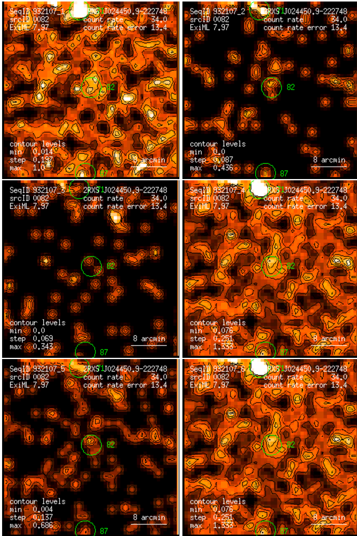
Figure 82: RASS 932107: detection 0082: band rate images, Gaussian filter: (1) PSPC channels 11 – 41, (2) 52 – 90, (3) 91 – 201, (4) 11 – 235, (5) 52 – 201, (6) 11 – 201. Broad band rates in counts/ks. Band rate contour levels in counts/ks/arcmin 2 .
