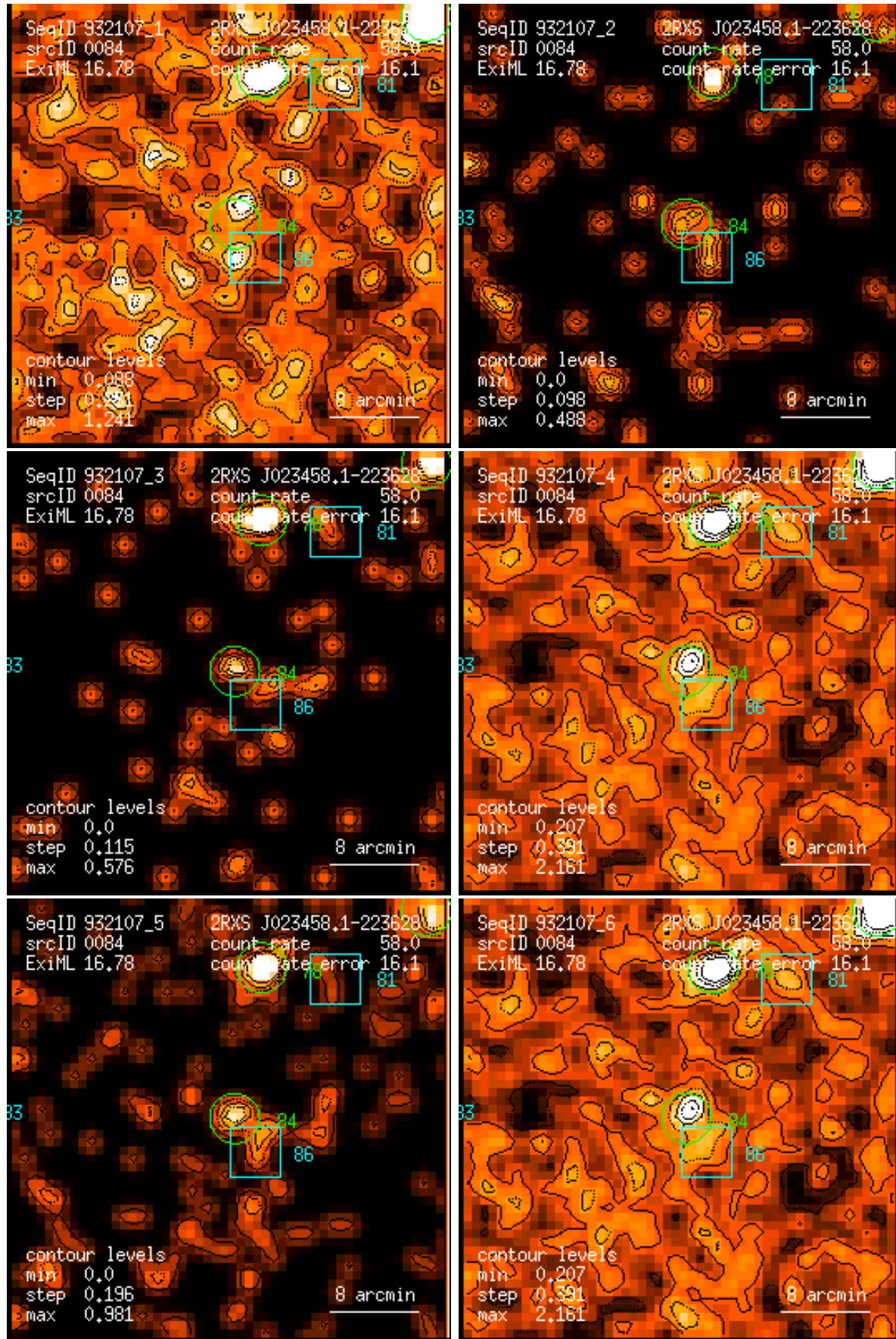
Figure 84: RASS 932107: detection 0084: band rate images, Gaussian filter: (1) PSPC channels 11 – 41, (2) 52 – 90, (3) 91 – 201, (4) 11 – 235, (5) 52 – 201, (6) 11 – 201. Broad band rates in counts/ks. Band rate contour levels in counts/ks/arcmin 2 .
