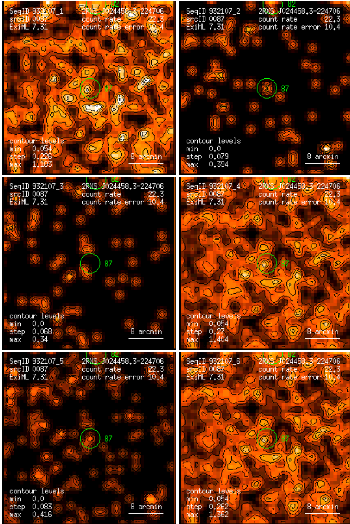
Figure 87: RASS 932107: detection 0087: band rate images, Gaussian filter: (1) PSPC channels 11 – 41, (2) 52 – 90, (3) 91 – 201, (4) 11 – 235, (5) 52 – 201, (6) 11 – 201. Broad band rates in counts/ks. Band rate contour levels in counts/ks/arcmin 2 .
