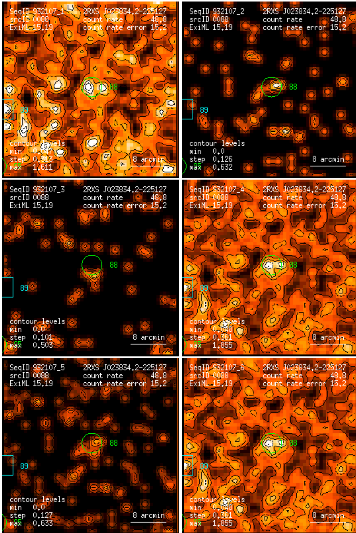
Figure 88: RASS 932107: detection 0088: band rate images, Gaussian filter: (1) PSPC channels 11 – 41, (2) 52 – 90, (3) 91 – 201, (4) 11 – 235, (5) 52 – 201, (6) 11 – 201. Broad band rates in counts/ks. Band rate contour levels in counts/ks/arcmin 2 .
