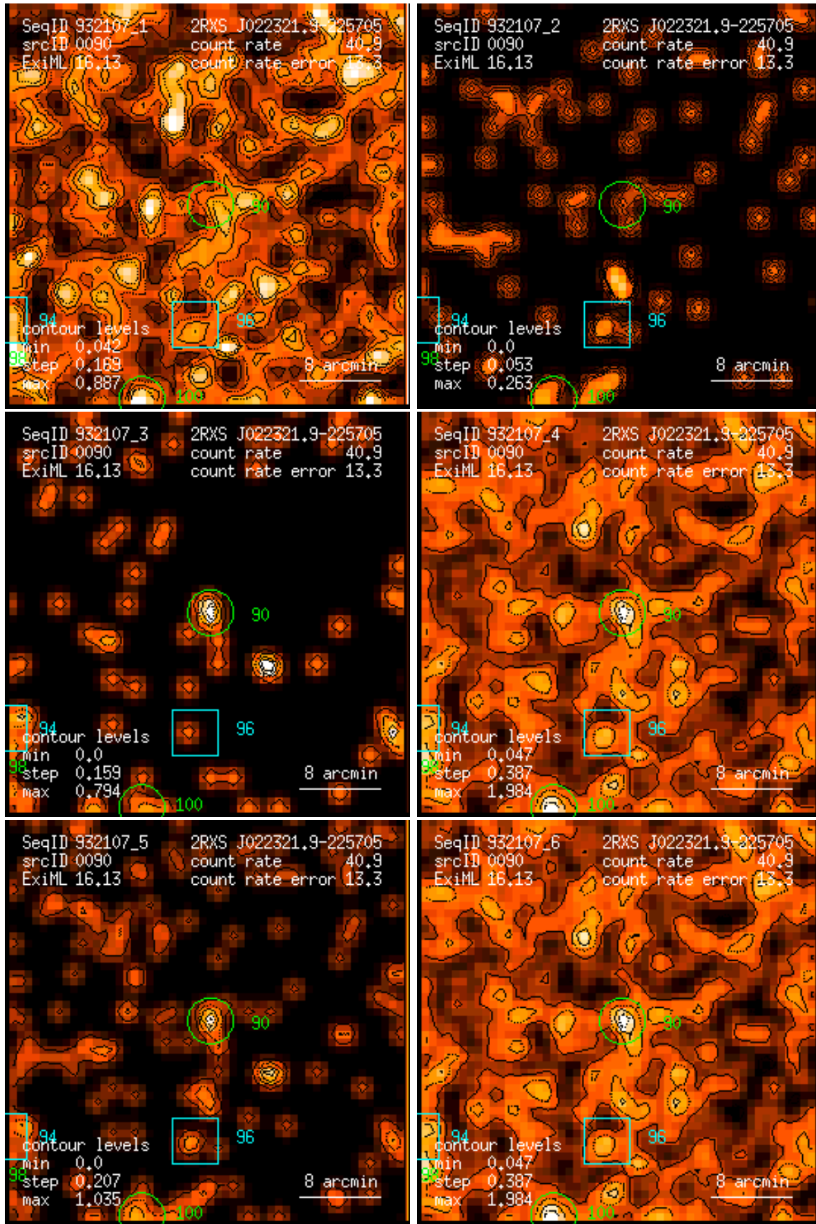
Figure 90: RASS 932107: detection 0090: band rate images, Gaussian filter: (1) PSPC channels 11 – 41, (2) 52 – 90, (3) 91 – 201, (4) 11 – 235, (5) 52 – 201, (6) 11 – 201. Broad band rates in counts/ks. Band rate contour levels in counts/ks/arcmin 2 .
