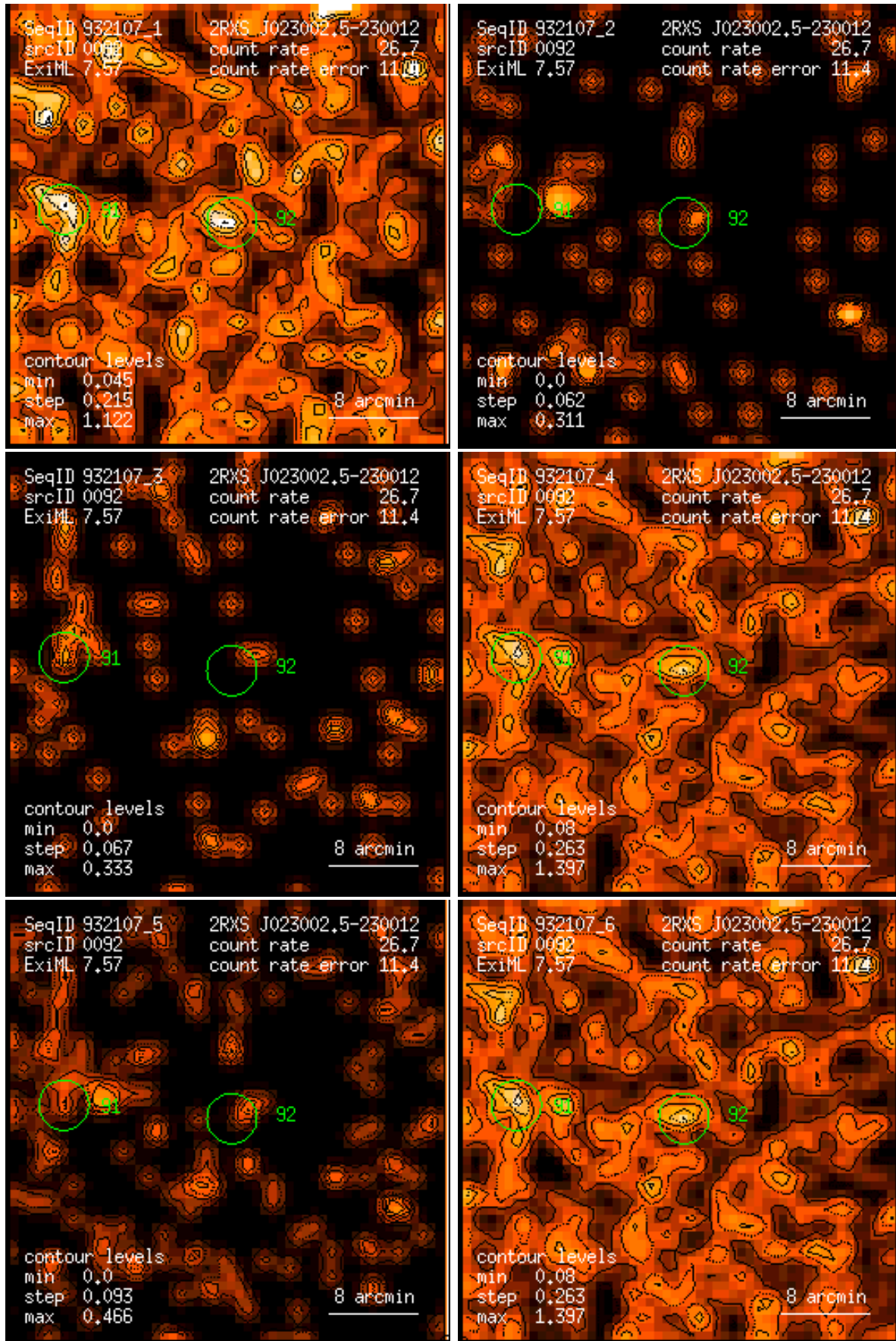
Figure 92: RASS 932107: detection 0092: band rate images, Gaussian filter: (1) PSPC channels 11 – 41, (2) 52 – 90, (3) 91 – 201, (4) 11 – 235, (5) 52 – 201, (6) 11 – 201. Broad band rates in counts/ks. Band rate contour levels in counts/ks/arcmin 2 .
