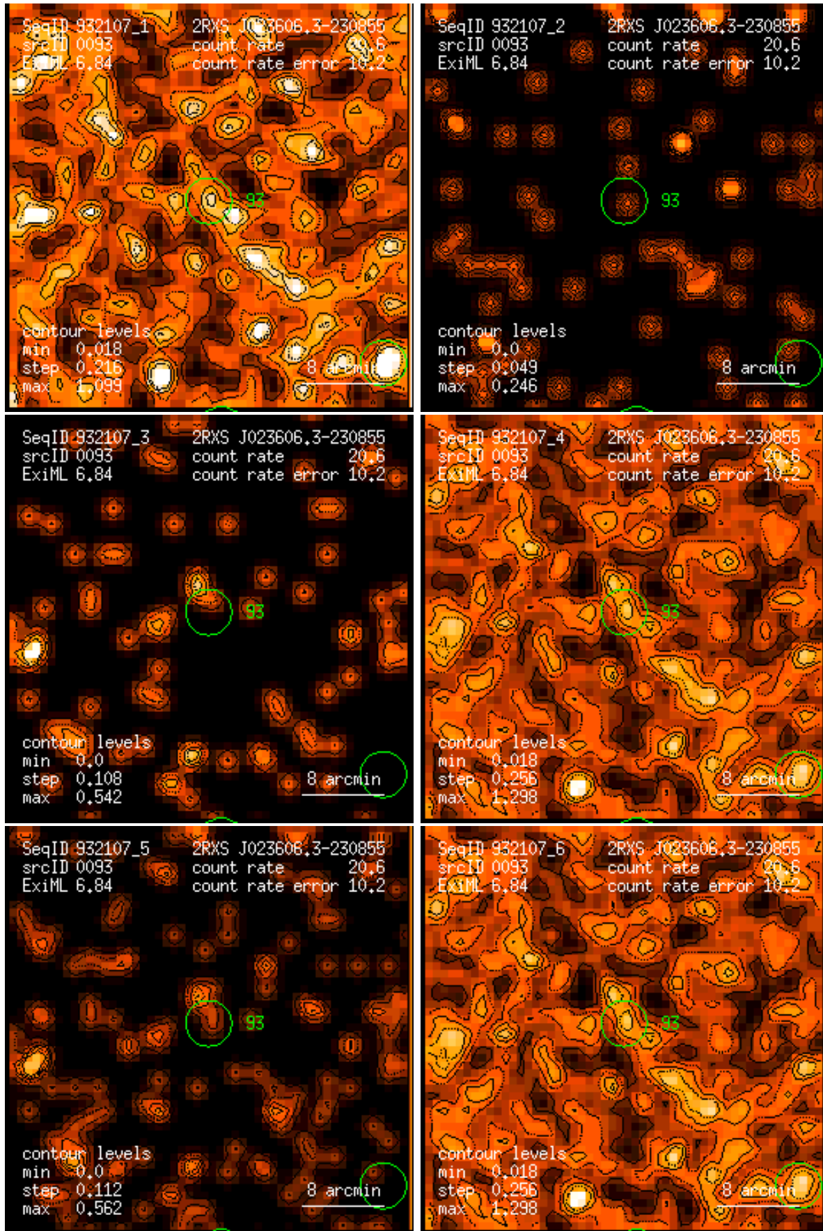
Figure 93: RASS 932107: detection 0093: band rate images, Gaussian filter: (1) PSPC channels 11 – 41, (2) 52 – 90, (3) 91 – 201, (4) 11 – 235, (5) 52 – 201, (6) 11 – 201. Broad band rates in counts/ks. Band rate contour levels in counts/ks/arcmin 2 .
