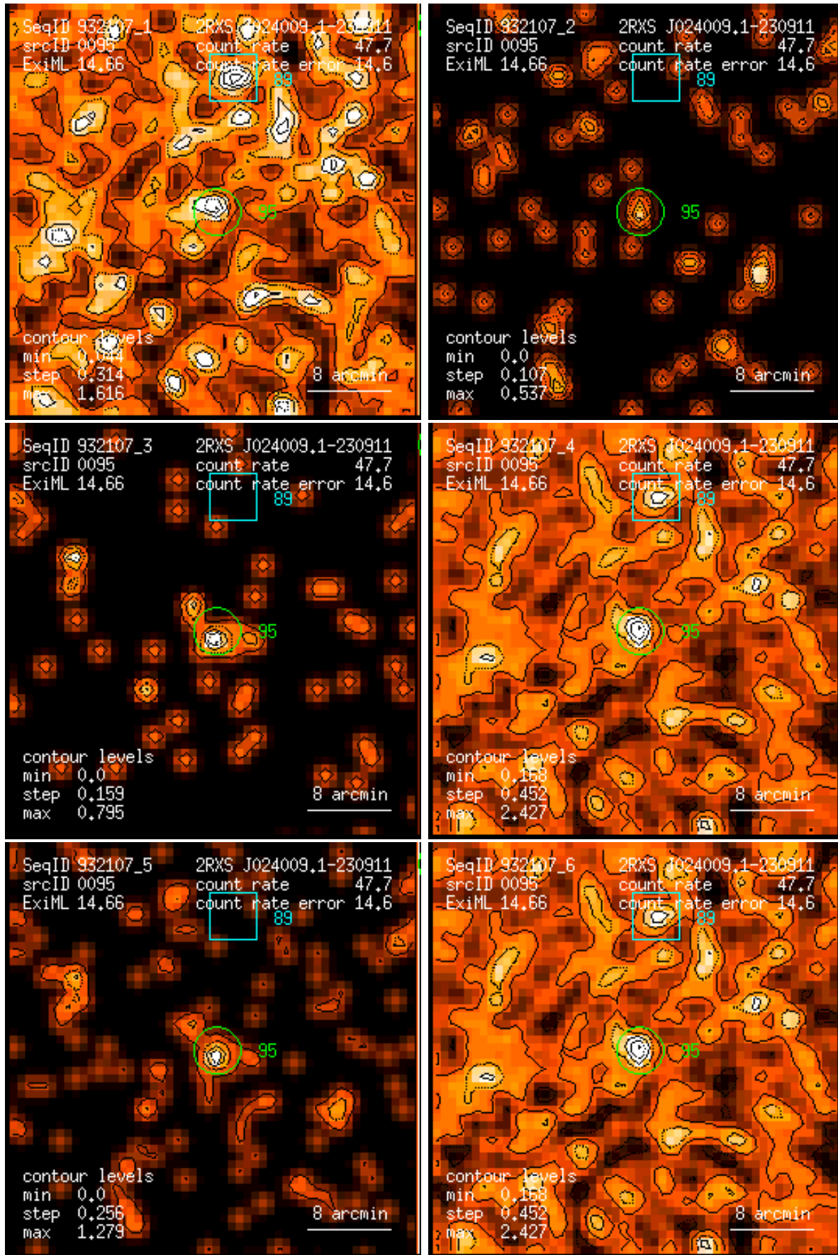
Figure 95: RASS 932107: detection 0095: band rate images, Gaussian filter: (1) PSPC channels 11 – 41, (2) 52 – 90, (3) 91 – 201, (4) 11 – 235, (5) 52 – 201, (6) 11 – 201. Broad band rates in counts/ks. Band rate contour levels in counts/ks/arcmin 2 .
