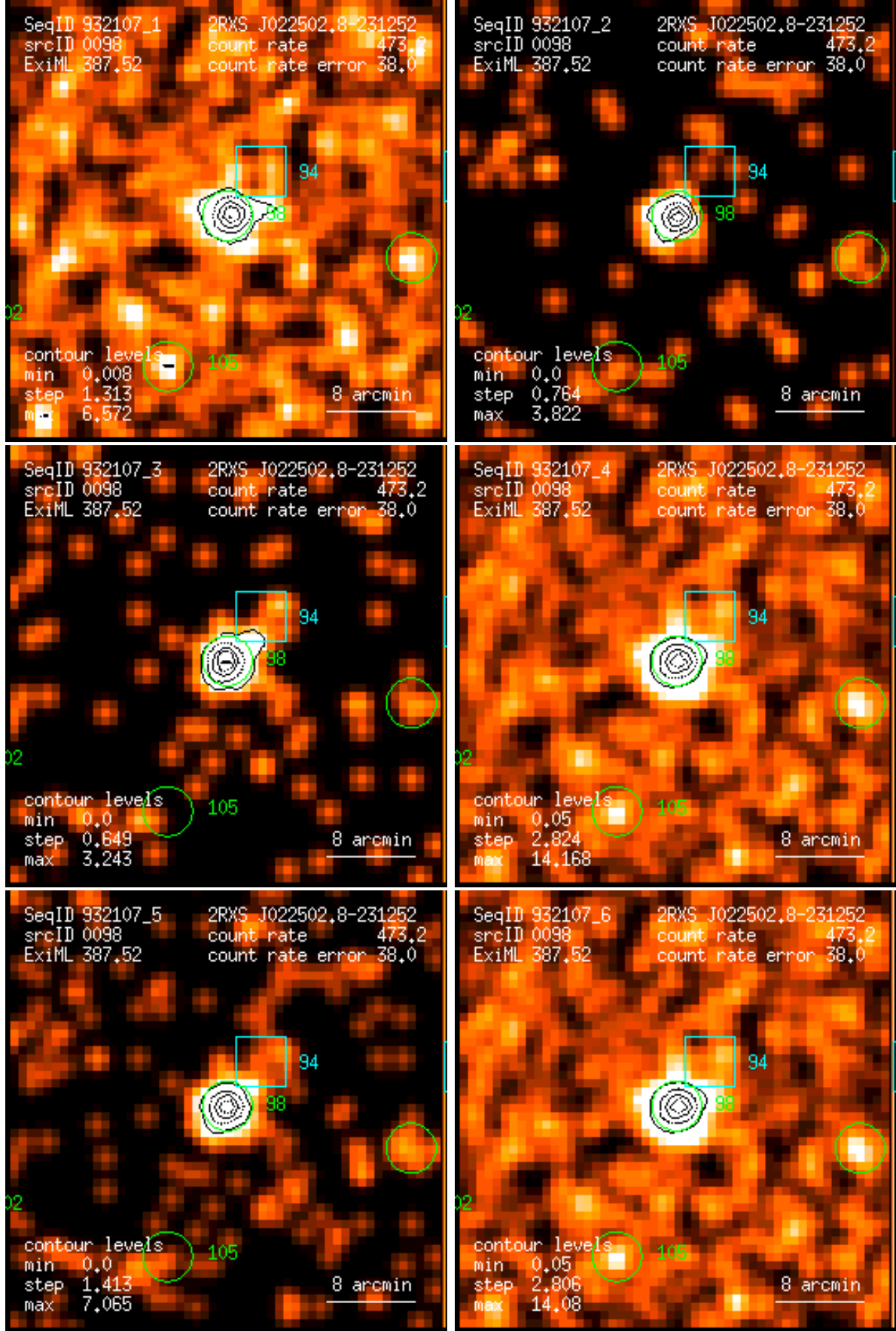
Figure 98: RASS 932107: detection 0098: band rate images, Gaussian filter: (1) PSPC channels 11 – 41, (2) 52 – 90, (3) 91 – 201, (4) 11 – 235, (5) 52 – 201, (6) 11 – 201. Broad band rates in counts/ks. Band rate contour levels in counts/ks/arcmin 2 .
