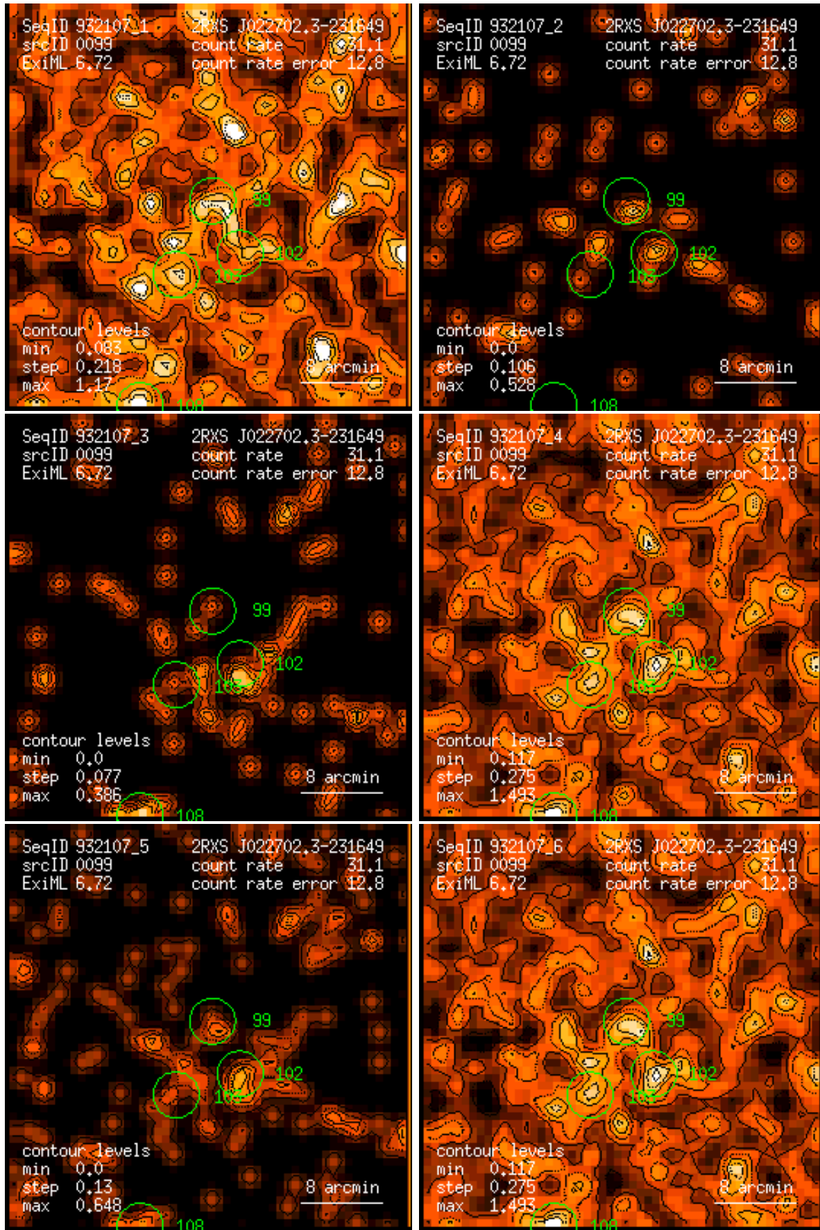
Figure 99: RASS 932107: detection 0099: band rate images, Gaussian filter: (1) PSPC channels 11 – 41, (2) 52 – 90, (3) 91 – 201, (4) 11 – 235, (5) 52 – 201, (6) 11 – 201. Broad band rates in counts/ks. Band rate contour levels in counts/ks/arcmin 2 .
