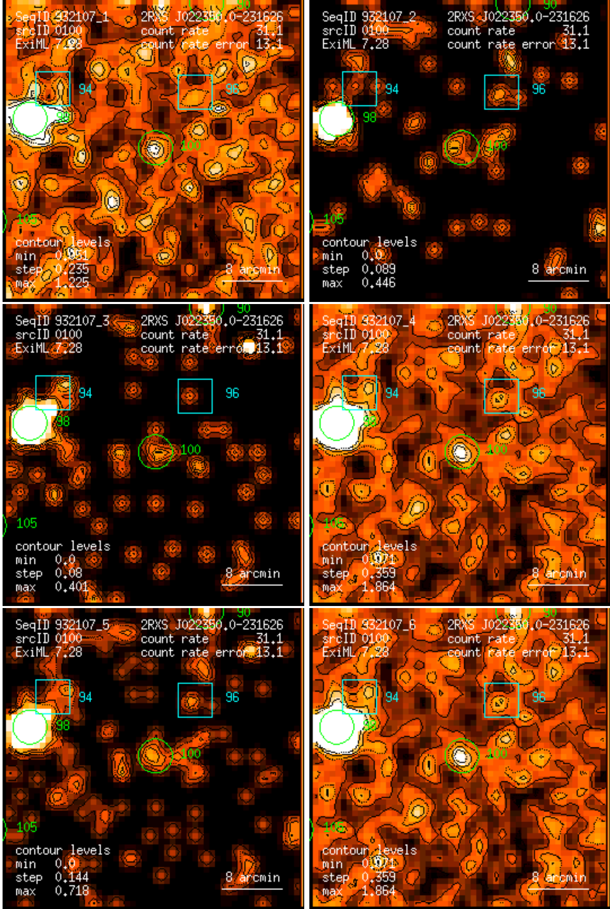
Figure 100: RASS 932107: detection 0100: band rate images, Gaussian filter: (1) PSPC channels 11 – 41, (2) 52 – 90, (3) 91 – 201, (4) 11 – 235, (5) 52 – 201, (6) 11 – 201. Broad band rates in counts/ks. Band rate contour levels in counts/ks/arcmin 2 .
