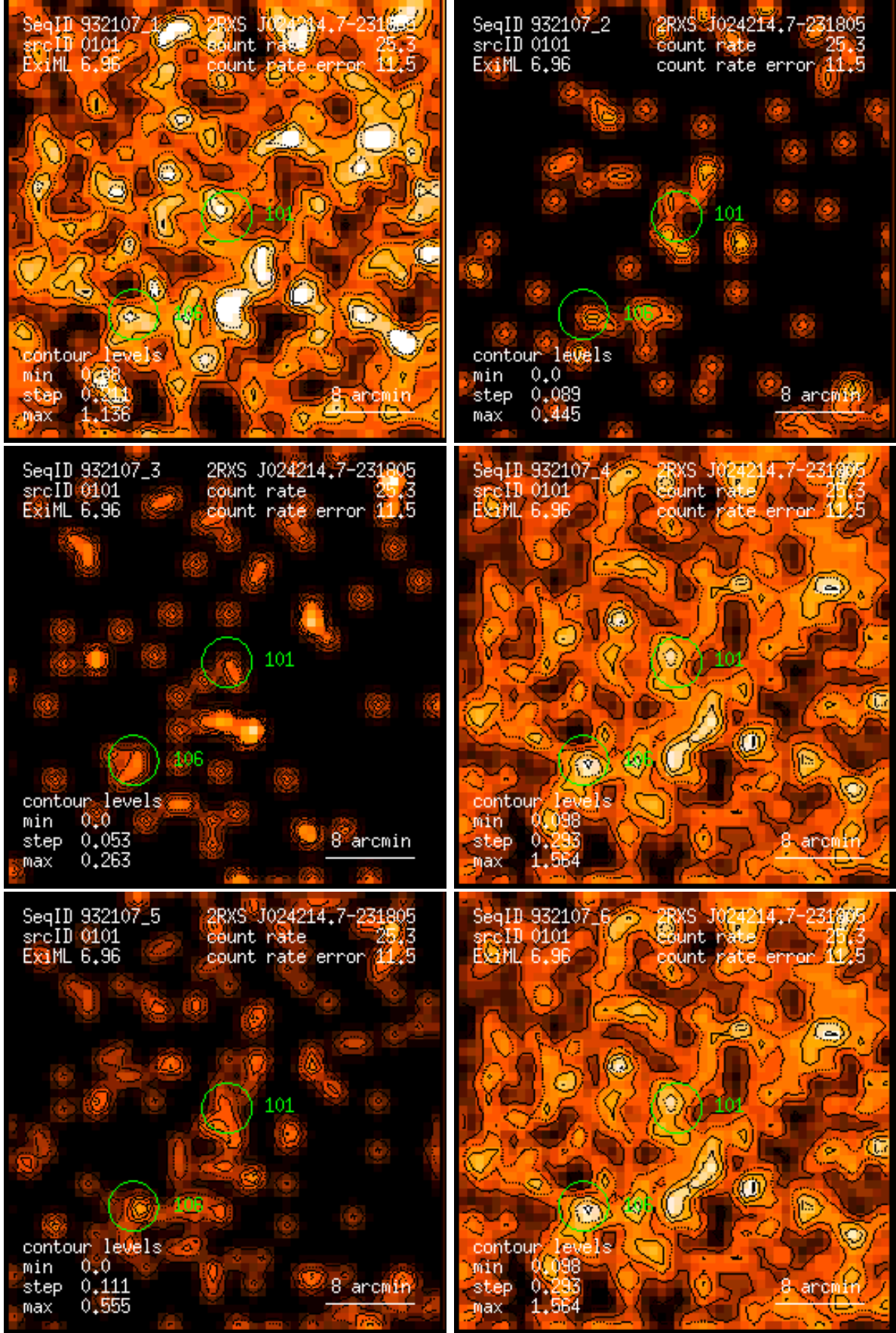
Figure 101: RASS 932107: detection 0101: band rate images, Gaussian filter: (1) PSPC channels 11 – 41, (2) 52 – 90, (3) 91 – 201, (4) 11 – 235, (5) 52 – 201, (6) 11 – 201. Broad band rates in counts/ks. Band rate contour levels in counts/ks/arcmin 2 .
