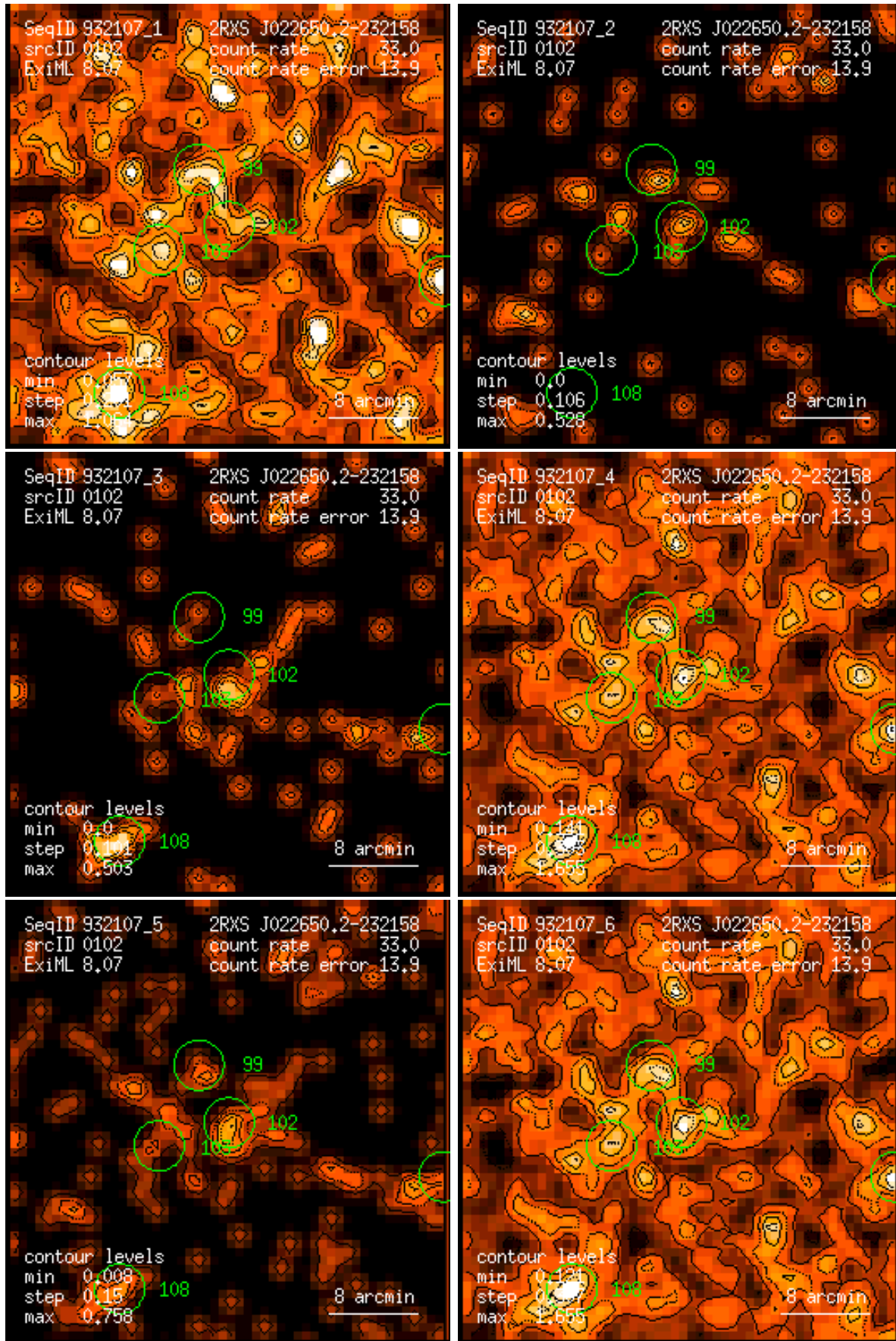
Figure 102: RASS 932107: detection 0102: band rate images, Gaussian filter: (1) PSPC channels 11 – 41, (2) 52 – 90, (3) 91 – 201, (4) 11 – 235, (5) 52 – 201, (6) 11 – 201. Broad band rates in counts/ks. Band rate contour levels in counts/ks/arcmin 2 .
