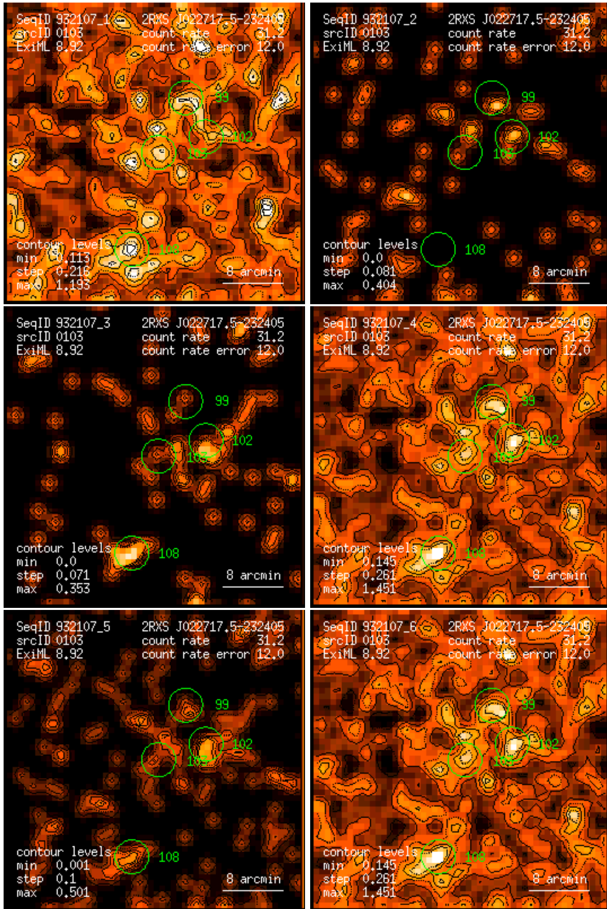
Figure 103: RASS 932107: detection 0103: band rate images, Gaussian filter: (1) PSPC channels 11 – 41, (2) 52 – 90, (3) 91 – 201, (4) 11 – 235, (5) 52 – 201, (6) 11 – 201. Broad band rates in counts/ks. Band rate contour levels in counts/ks/arcmin 2 .
