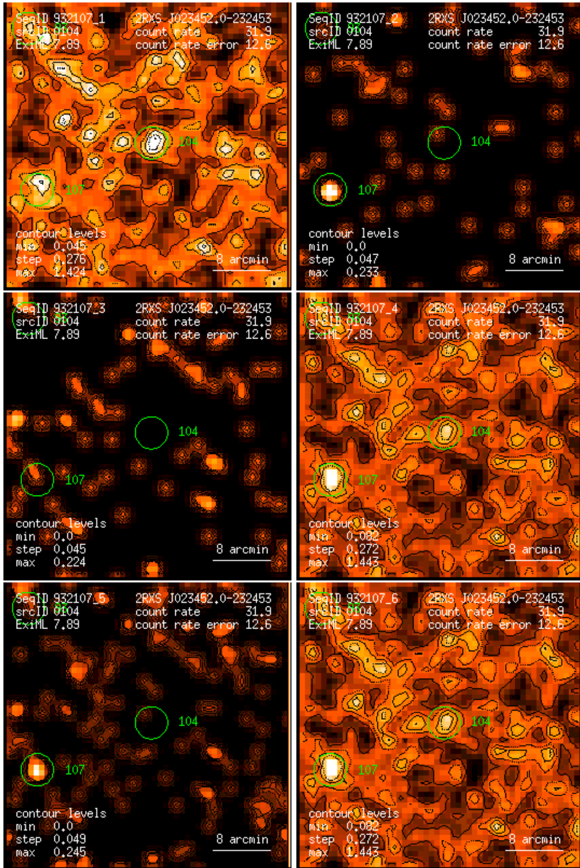
Figure 104: RASS 932107: detection 0104: band rate images, Gaussian filter: (1) PSPC channels 11 – 41, (2) 52 – 90, (3) 91 – 201, (4) 11 – 235, (5) 52 – 201, (6) 11 – 201. Broad band rates in counts/ks. Band rate contour levels in counts/ks/arcmin 2 .
