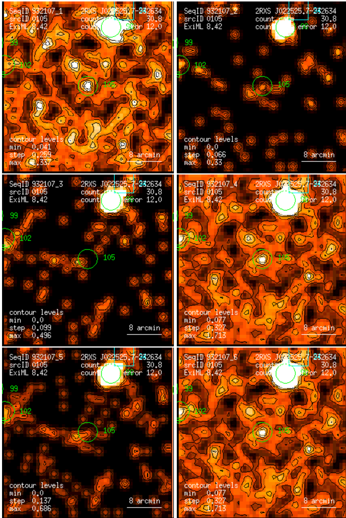
Figure 105: RASS 932107: detection 0105: band rate images, Gaussian filter: (1) PSPC channels 11 – 41, (2) 52 – 90, (3) 91 – 201, (4) 11 – 235, (5) 52 – 201, (6) 11 – 201. Broad band rates in counts/ks. Band rate contour levels in counts/ks/arcmin 2 .
