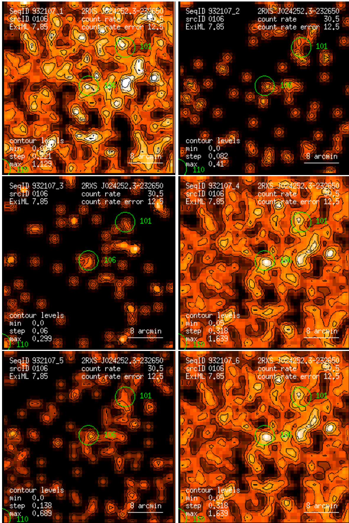
Figure 106: RASS 932107: detection 0106: band rate images, Gaussian filter: (1) PSPC channels 11 – 41, (2) 52 – 90, (3) 91 – 201, (4) 11 – 235, (5) 52 – 201, (6) 11 – 201. Broad band rates in counts/ks. Band rate contour levels in counts/ks/arcmin 2 .
