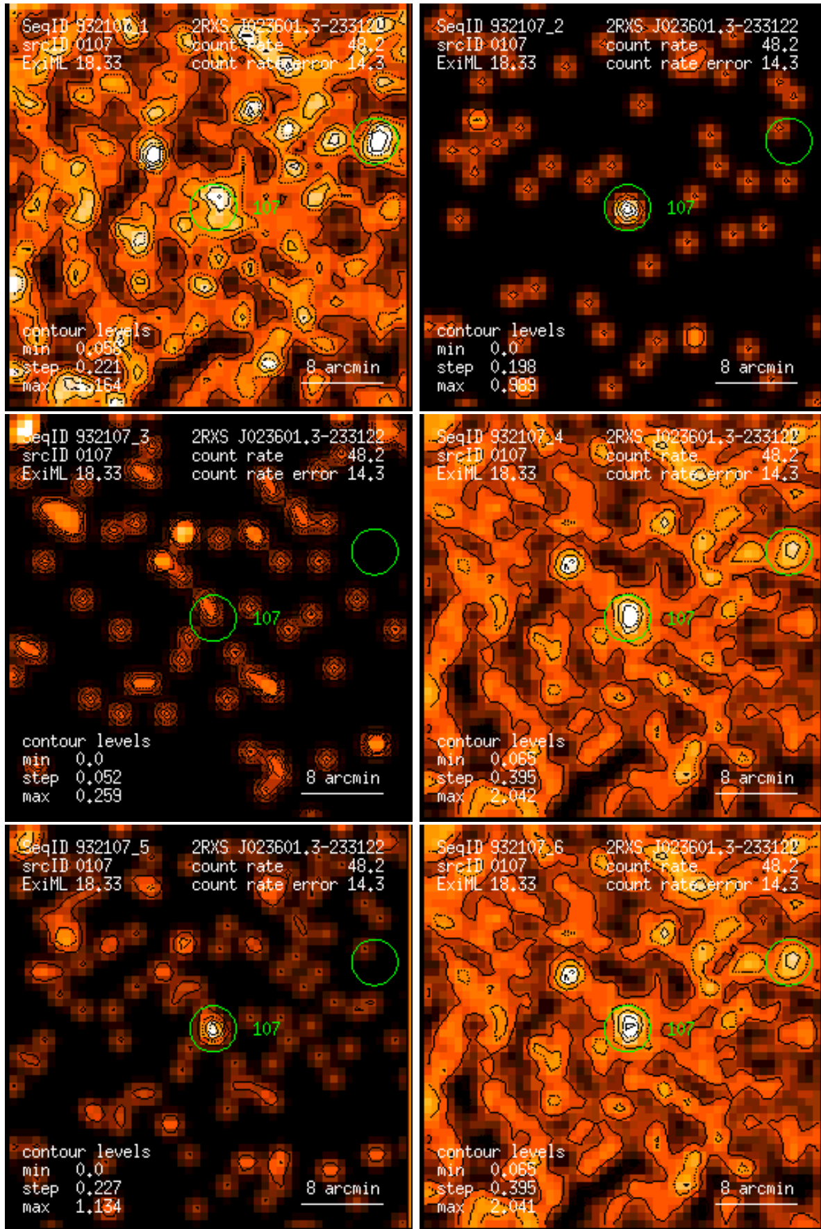
Figure 107: RASS 932107: detection 0107: band rate images, Gaussian filter: (1) PSPPC channels 11 – 41, (2) 52 – 90, (3) 91 – 201, (4) 11 – 235, (5) 52 – 201, (6) 11 – 201. Broad band rates in counts/ks. Band rate contour levels in counts/ks/arcmin 2 .
