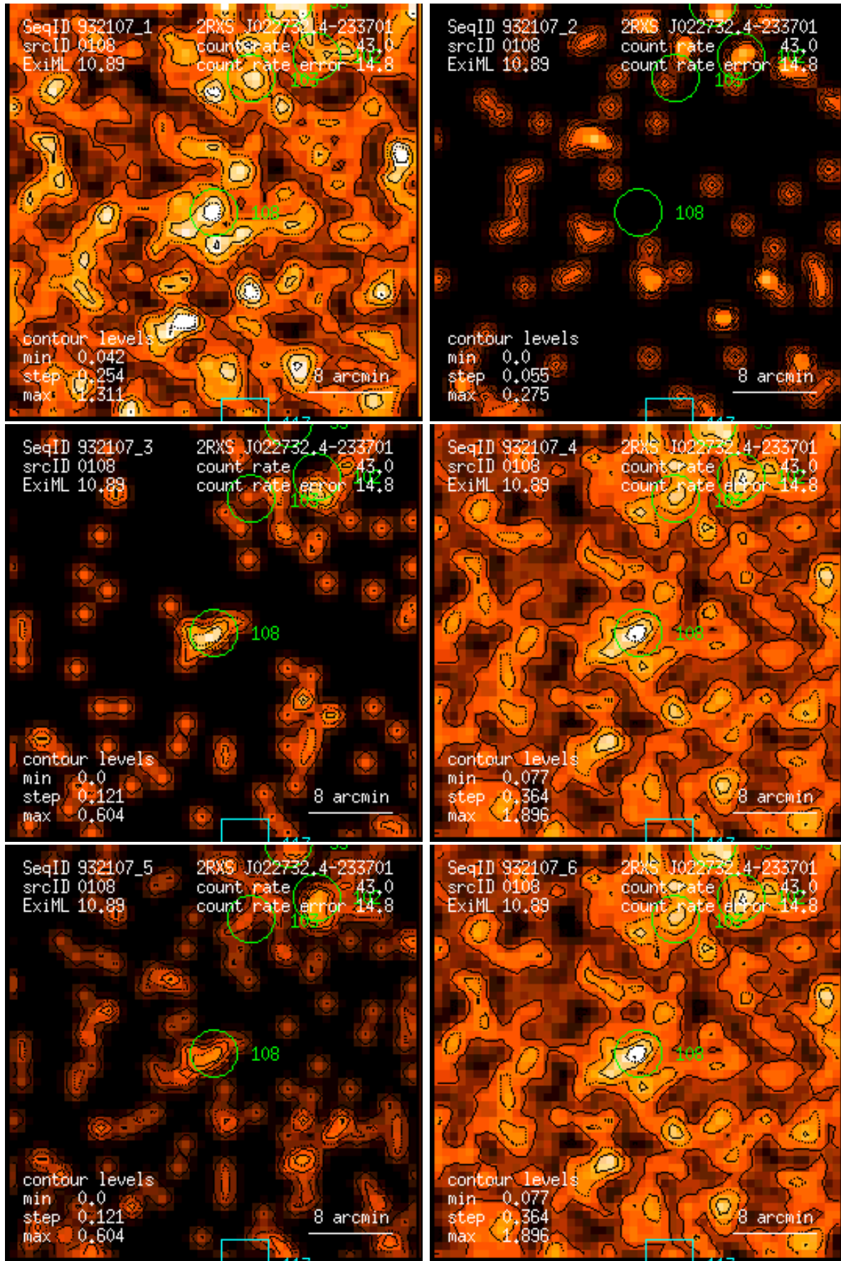
Figure 108: RASS 932107: detection 0108: band rate images, Gaussian filter: (1) PSPC channels 11 – 41, (2) 52 – 90, (3) 91 – 201, (4) 11 – 235, (5) 52 – 201, (6) 11 – 201. Broad band rates in counts/ks. Band rate contour levels in counts/ks/arcmin 2 .
