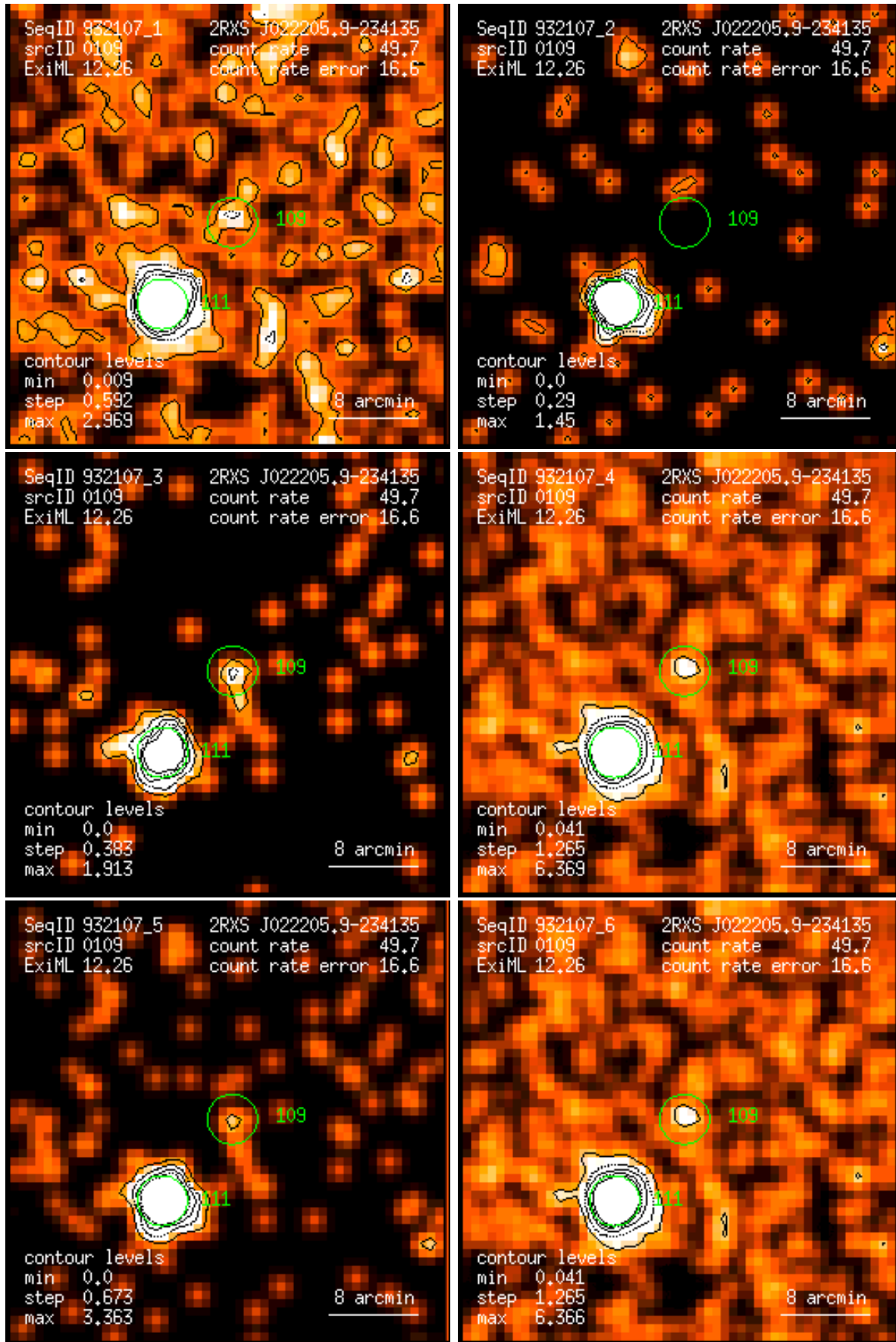
Figure 109: RASS 932107: detection 0109: band rate images, Gaussian filter: (1) PSPC channels 11 – 41, (2) 52 – 90, (3) 91 – 201, (4) 11 – 235, (5) 52 – 201, (6) 11 – 201. Broad band rates in counts/ks. Band rate contour levels in counts/ks/arcmin 2 .
