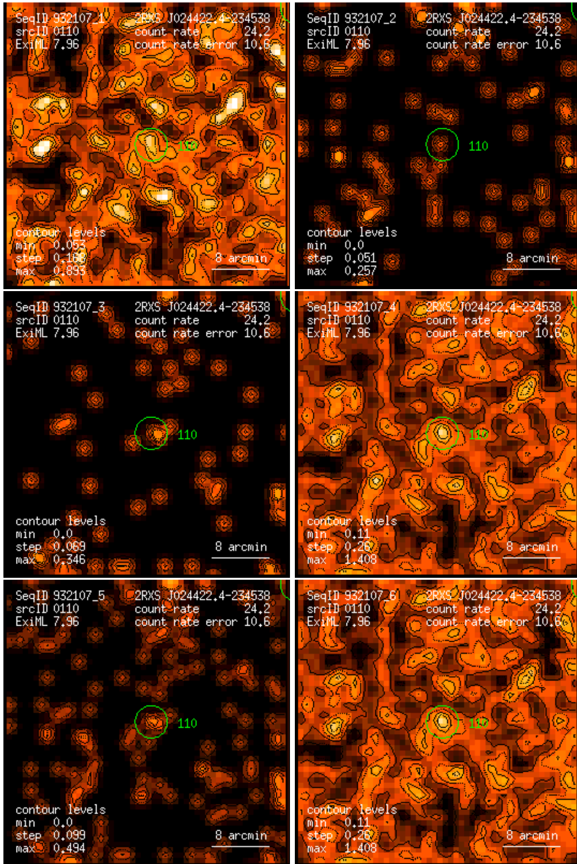
Figure 110: RASS 932107: detection 0110: band rate images, Gaussian filter: (1) PSPC channels 11 – 41, (2) 52 – 90, (3) 91 – 201, (4) 11 – 235, (5) 52 – 201, (6) 11 – 201. Broad band rates in counts/ks. Band rate contour levels in counts/ks/arcmin 2 .
