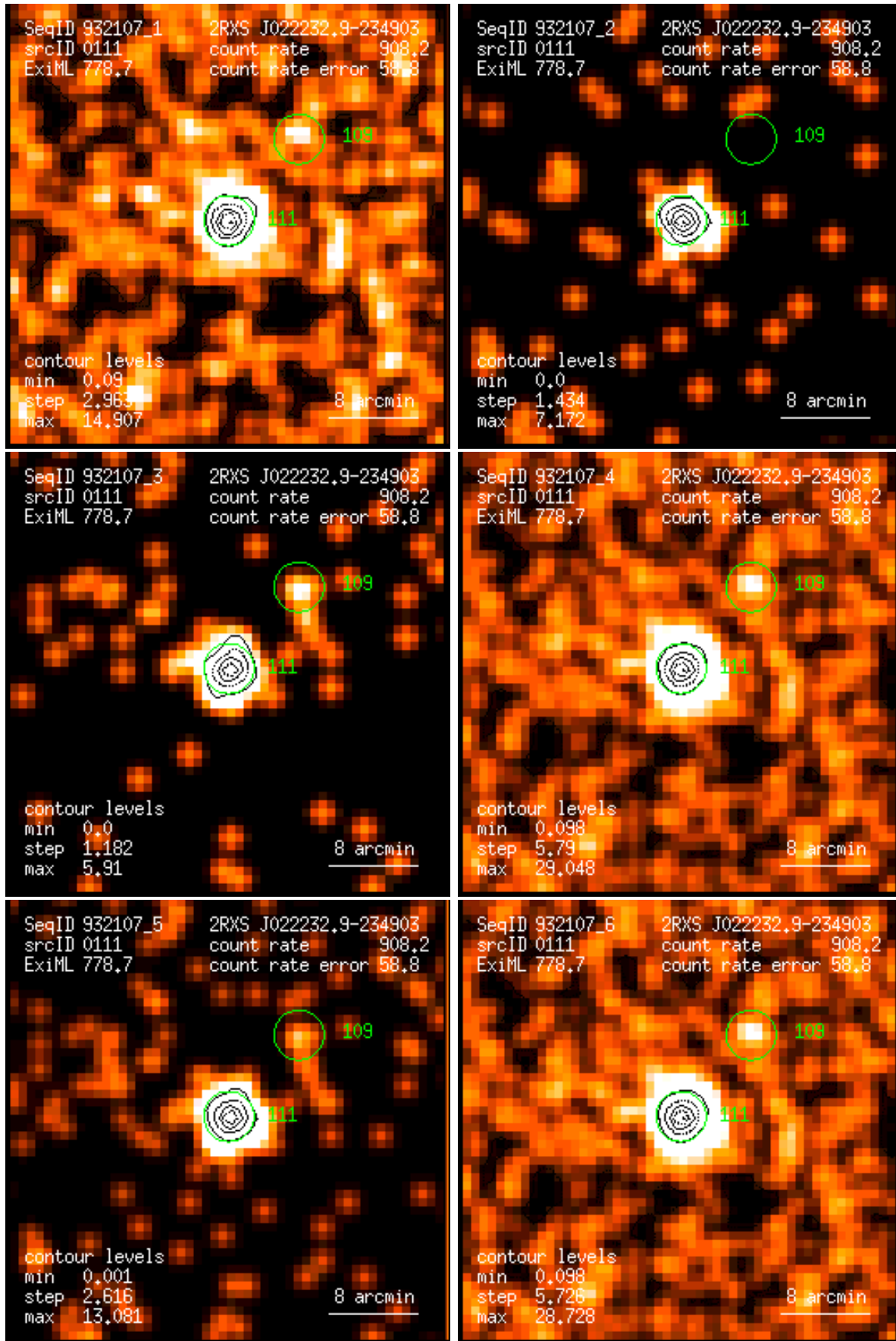
Figure 111: RASS 932107: detection 0111: band rate images, Gaussian filter: (1) PSPC channels 11 – 41, (2) 52 – 90, (3) 91 – 201, (4) 11 – 235, (5) 52 – 201, (6) 11 – 201. Broad band rates in counts/ks. Band rate contour levels in counts/ks/arcmin 2 .
