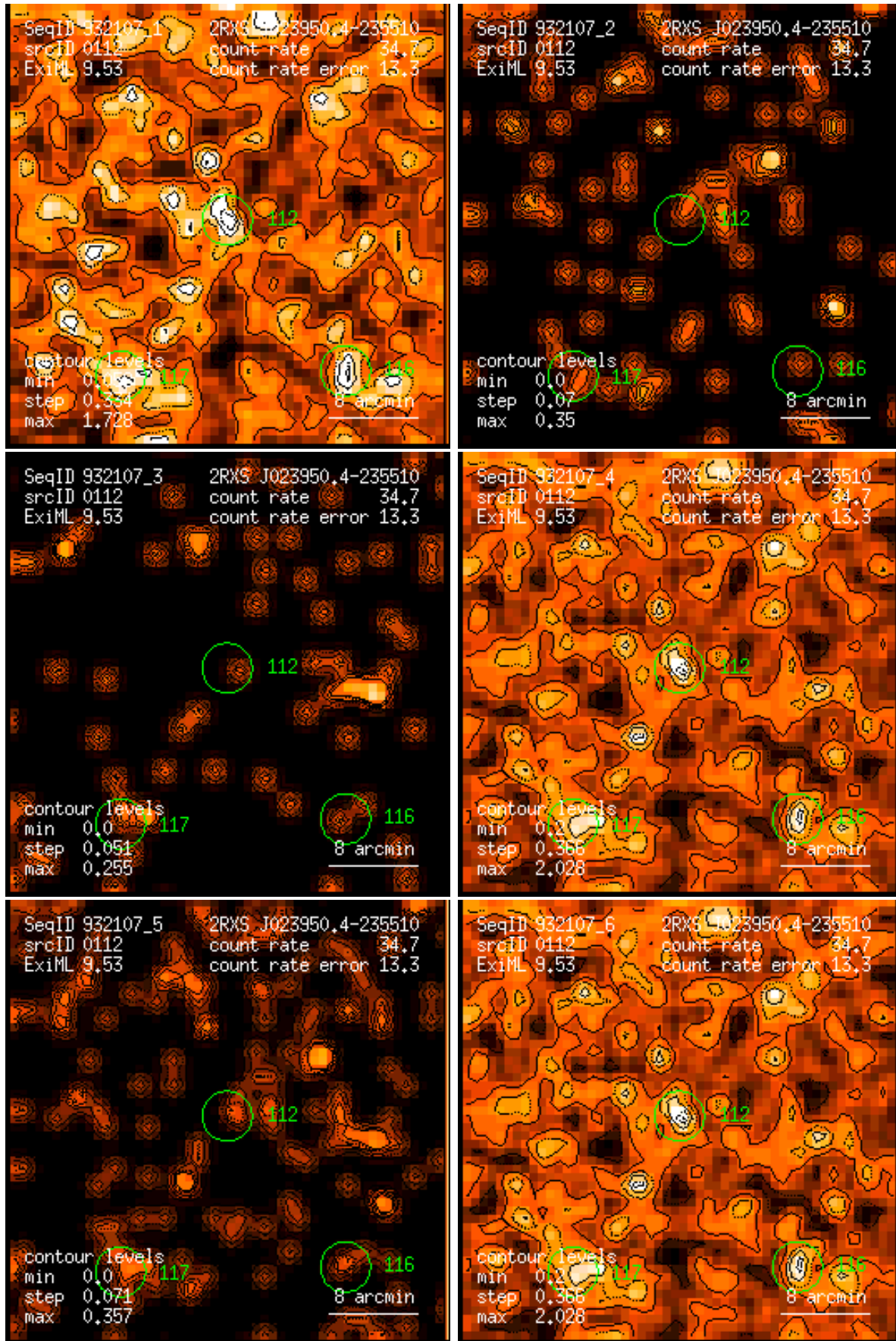
Figure 112: RASS 932107: detection 0112: band rate images, Gaussian filter: (1) PSPC channels 11 – 41, (2) 52 – 90, (3) 91 – 201, (4) 11 – 235, (5) 52 – 201, (6) 11 – 201. Broad band rates in counts/ks. Band rate contour levels in counts/ks/arcmin 2 .
