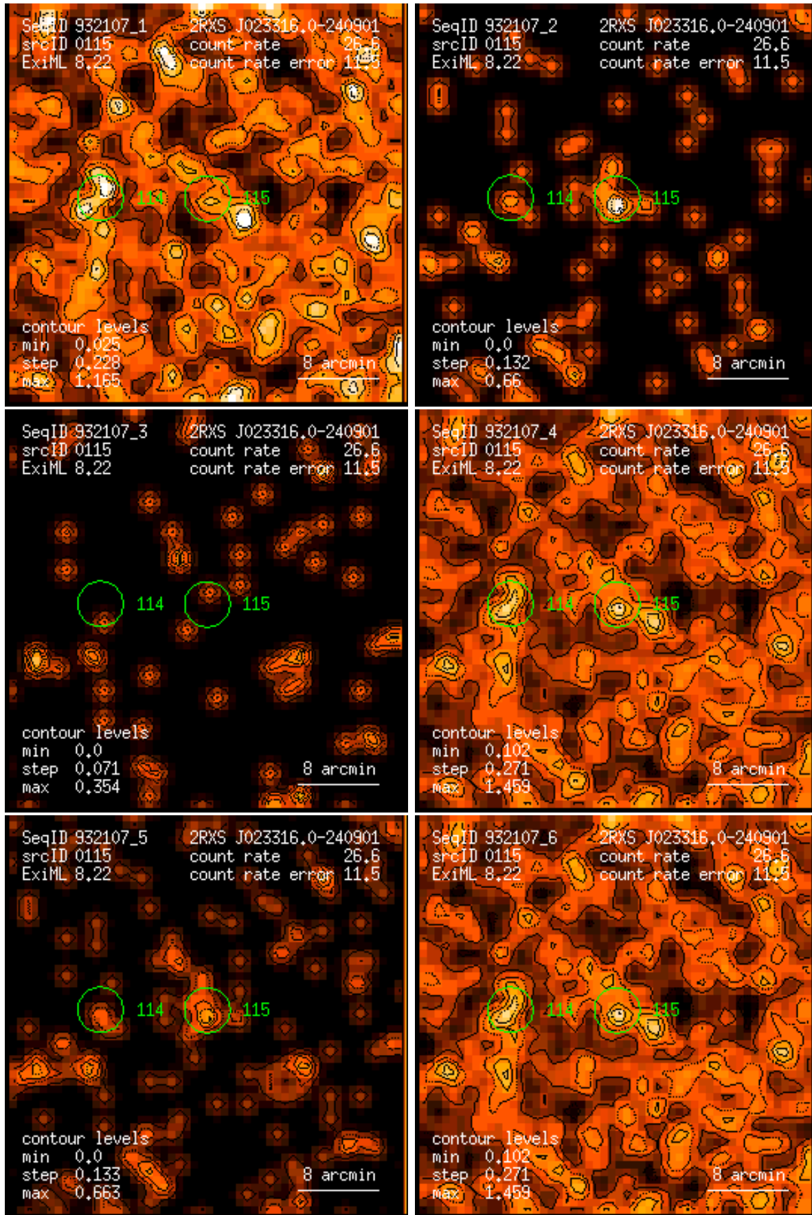
Figure 115: RASS 932107: detection 0115: band rate images, Gaussian filter: (1) PSPC channels 11 – 41, (2) 52 – 90, (3) 91 – 201, (4) 11 – 235, (5) 52 – 201, (6) 11 – 201. Broad band rates in counts/ks. Band rate contour levels in counts/ks/arcmin 2 .
