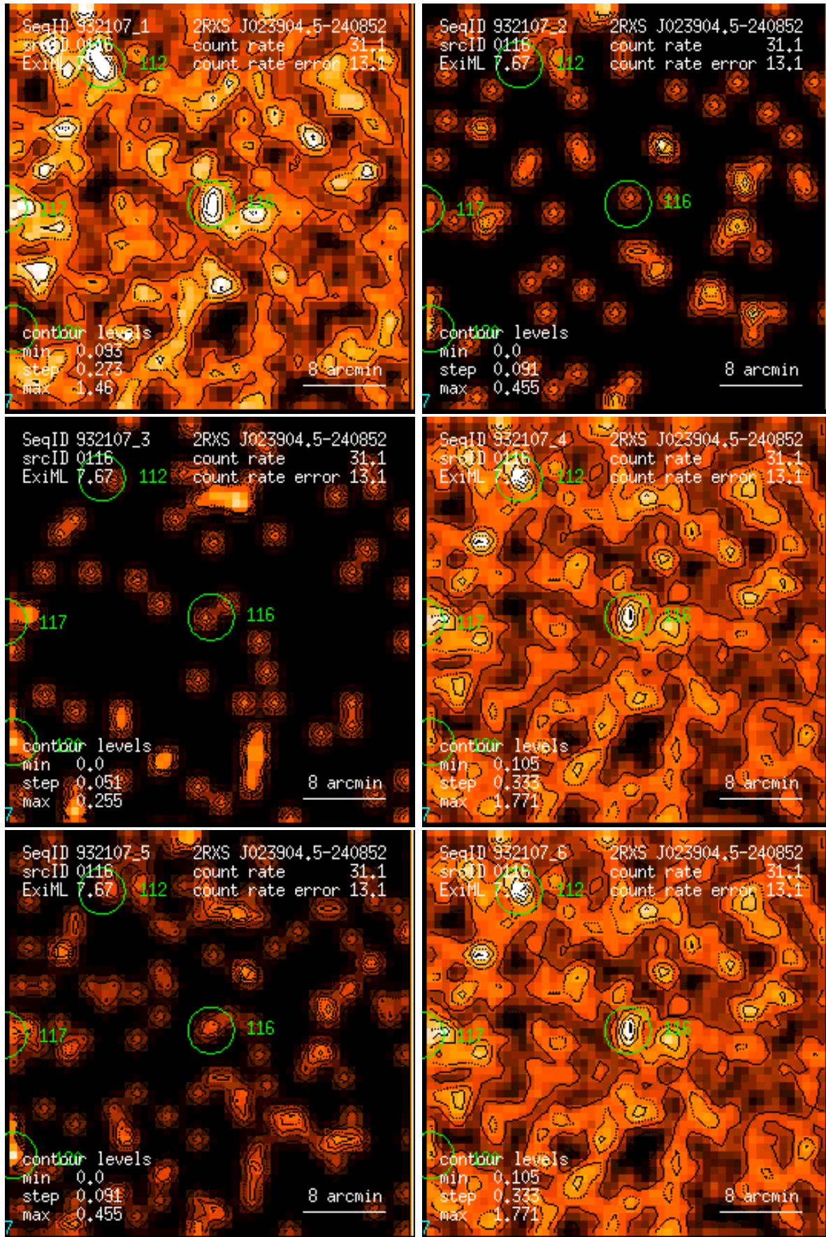
Figure 116: RASS 932107: detection 0116: band rate images, Gaussian filter: (1) PSPC channels 11 – 41, (2) 52 – 90, (3) 91 – 201, (4) 11 – 235, (5) 52 – 201, (6) 11 – 201. Broad band rates in counts/ks. Band rate contour levels in counts/ks/arcmin 2 .
