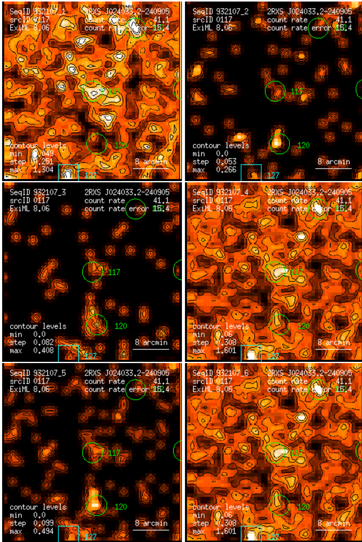
Figure 117: RASS 932107: detection 0117: band rate images, Gaussian filter: (1) PSPC channels 11 – 41, (2) 52 – 90, (3) 91 – 201, (4) 11 – 235, (5) 52 – 201, (6) 11 – 201. Broad band rates in counts/ks. Band rate contour levels in counts/ks/arcmin 2 .
