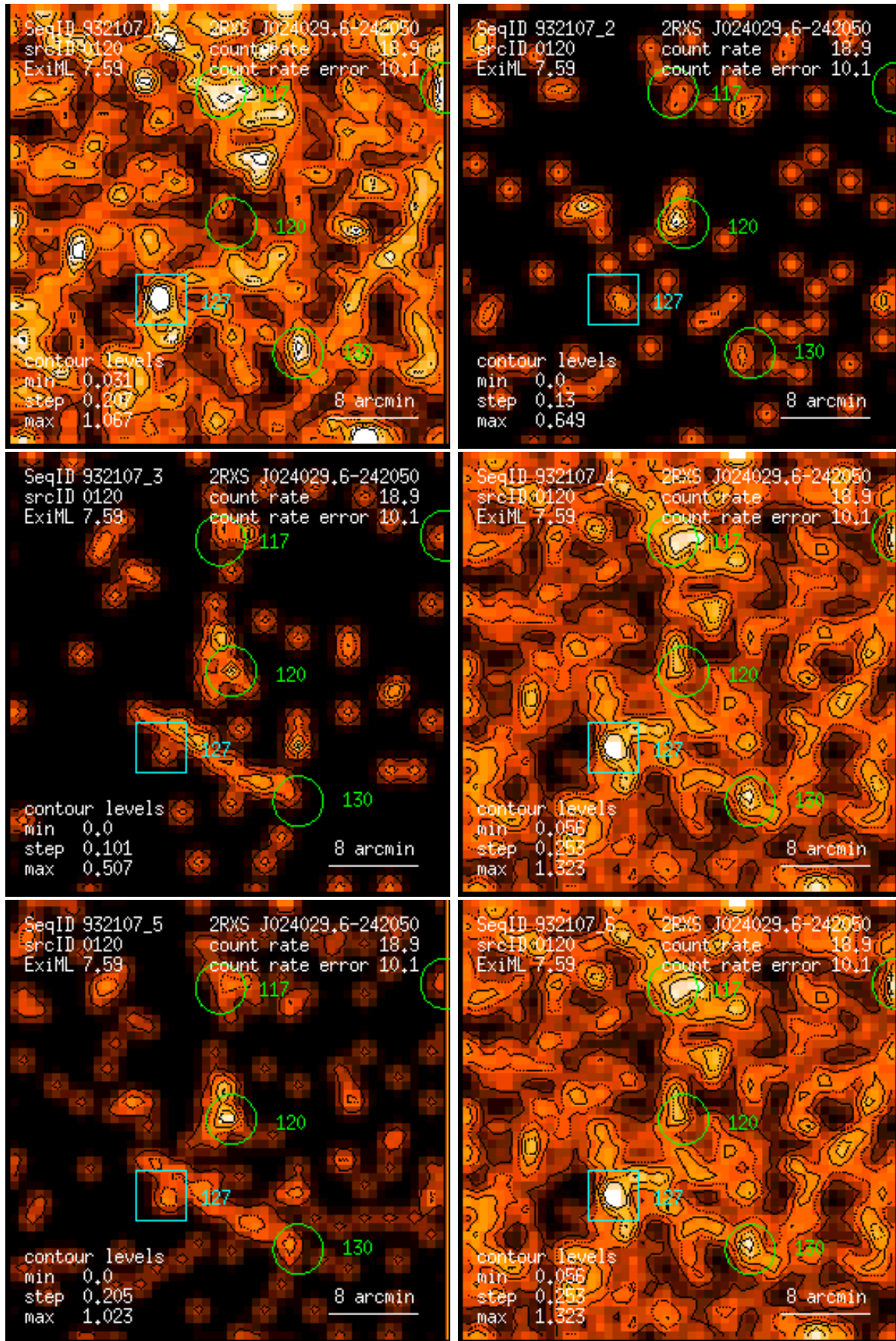
Figure 120: RASS 932107: detection 0120: band rate images, Gaussian filter: (1) PSPC channels 11 – 41, (2) 52 – 90, (3) 91 – 201, (4) 11 – 235, (5) 52 – 201, (6) 11 – 201. Broad band rates in counts/ks. Band rate contour levels in counts/ks/arcmin 2 .
