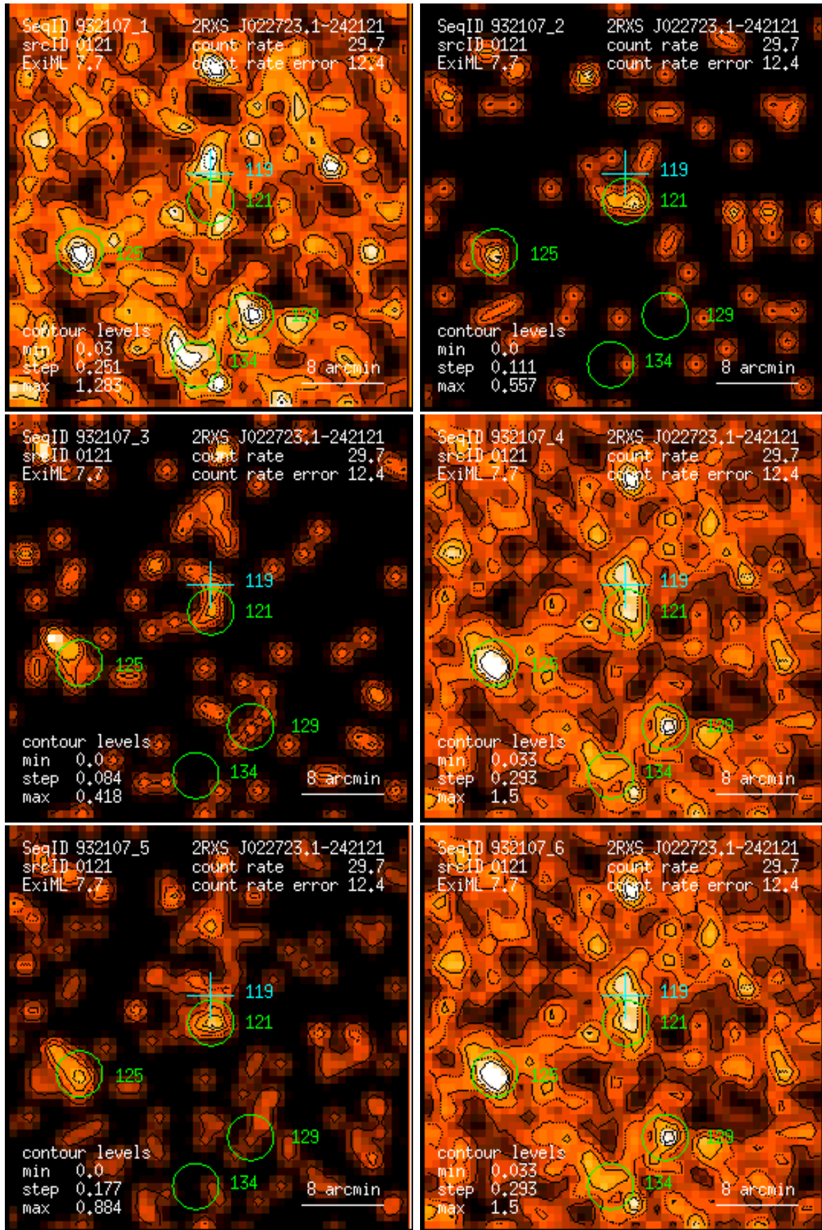
Figure 121: RASS 932107: detection 0121: band rate images, Gaussian filter: (1) PSPC channels 11 – 41, (2) 52 – 90, (3) 91 – 201, (4) 11 – 235, (5) 52 – 201, (6) 11 – 201. Broad band rates in counts/ks. Band rate contour levels in counts/ks/arcmin 2 .
