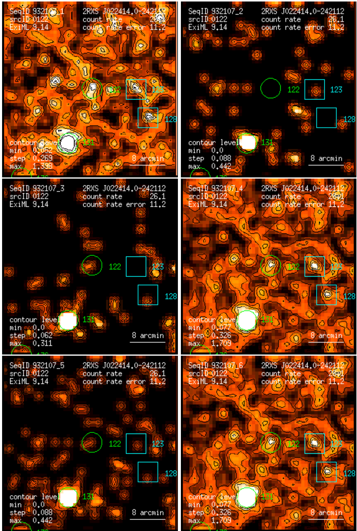
Figure 122: RASS 932107: detection 0122: band rate images, Gaussian filter: (1) PSPC channels 11 – 41, (2) 52 – 90, (3) 91 – 201, (4) 11 – 235, (5) 52 – 201, (6) 11 – 201. Broad band rates in counts/ks. Band rate contour levels in counts/ks/arcmin 2 .
