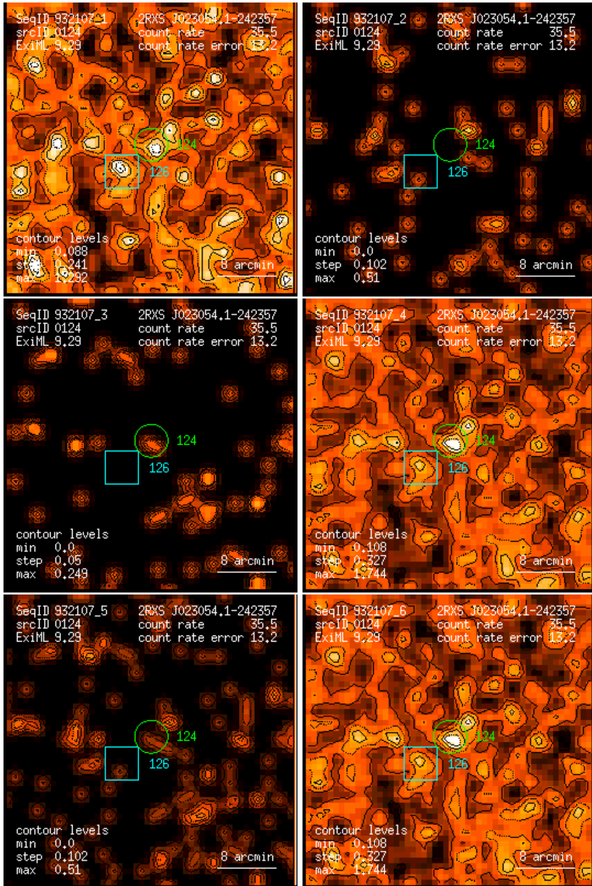
Figure 124: RASS 932107: detection 0124: band rate images, Gaussian filter: (1) PSPC channels 11 – 41, (2) 52 – 90, (3) 91 – 201, (4) 11 – 235, (5) 52 – 201, (6) 11 – 201. Broad band rates in counts/ks. Band rate contour levels in counts/ks/arcmin 2 .
