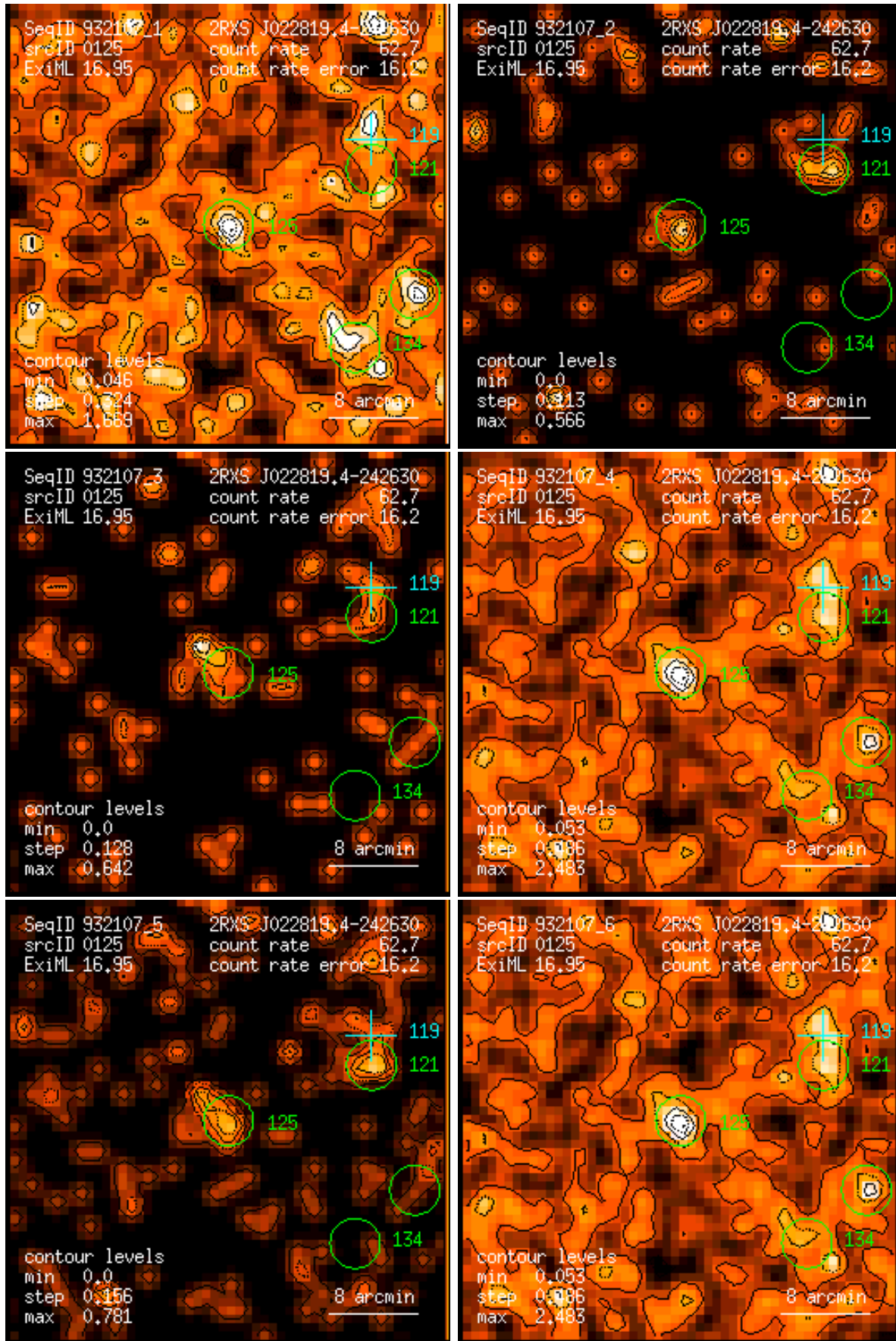
Figure 125: RASS 932107: detection 0125: band rate images, Gaussian filter: (1) PSPC channels 11 – 41, (2) 52 – 90, (3) 91 – 201, (4) 11 – 235, (5) 52 – 201, (6) 11 – 201. Broad band rates in counts/ks. Band rate contour levels in counts/ks/arcmin 2 .
