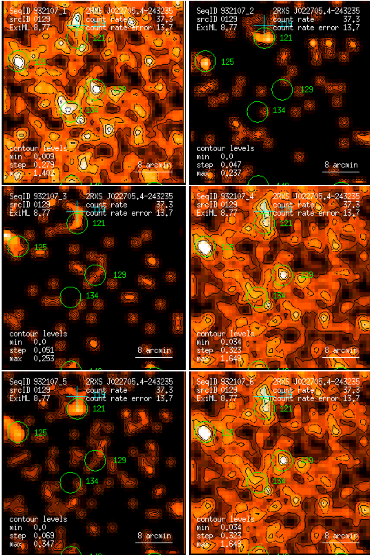
Figure 129: RASS 932107: detection 0129: band rate images, Gaussian filter: (1) PSPC channels 11 – 41, (2) 52 – 90, (3) 91 – 201, (4) 11 – 235, (5) 52 – 201, (6) 11 – 201. Broad band rates in counts/ks. Band rate contour levels in counts/ks/arcmin 2 .
