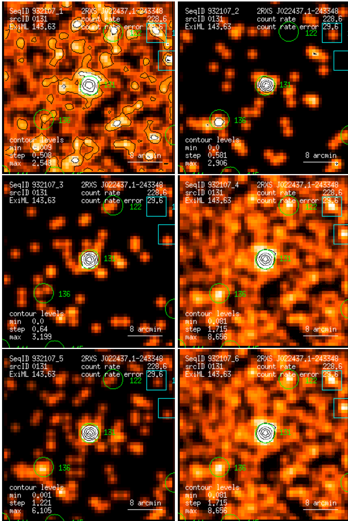
Figure 131: RASS 932107: detection 0131: band rate images, Gaussian filter: (1) PSPC channels 11 – 41, (2) 52 – 90, (3) 91 – 201, (4) 11 – 235, (5) 52 – 201, (6) 11 – 201. Broad band rates in counts/ks. Band rate contour levels in counts/ks/arcmin 2 .
