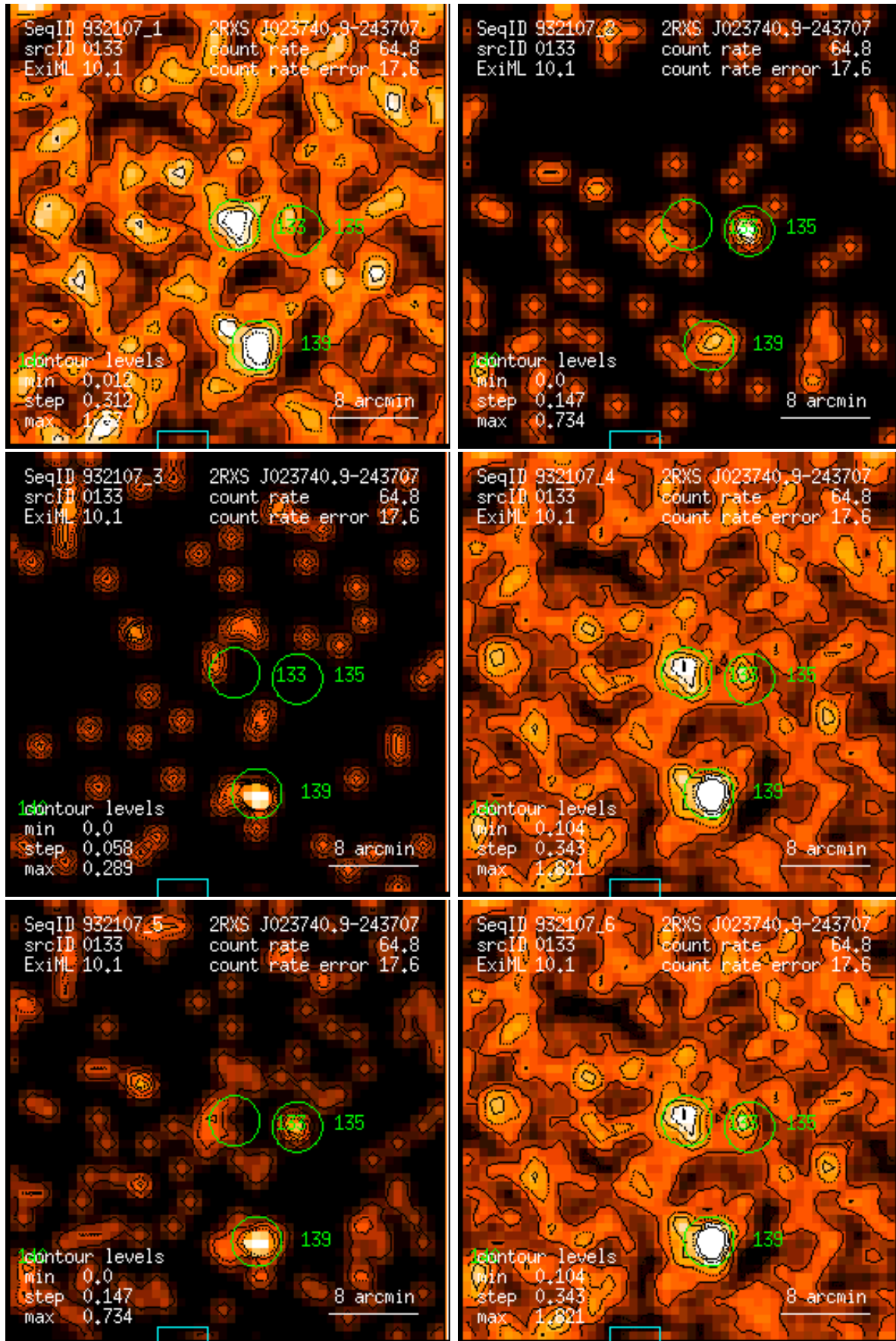
Figure 133: RASS 932107: detection 0133: band rate images, Gaussian filter: (1) PSPC channels 11 – 41, (2) 52 – 90, (3) 91 – 201, (4) 11 – 235, (5) 52 – 201, (6) 11 – 201. Broad band rates in counts/ks. Band rate contour levels in counts/ks/arcmin 2 .
